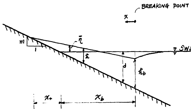
Figure D-1 Definition Sketch of Wave Set-up
