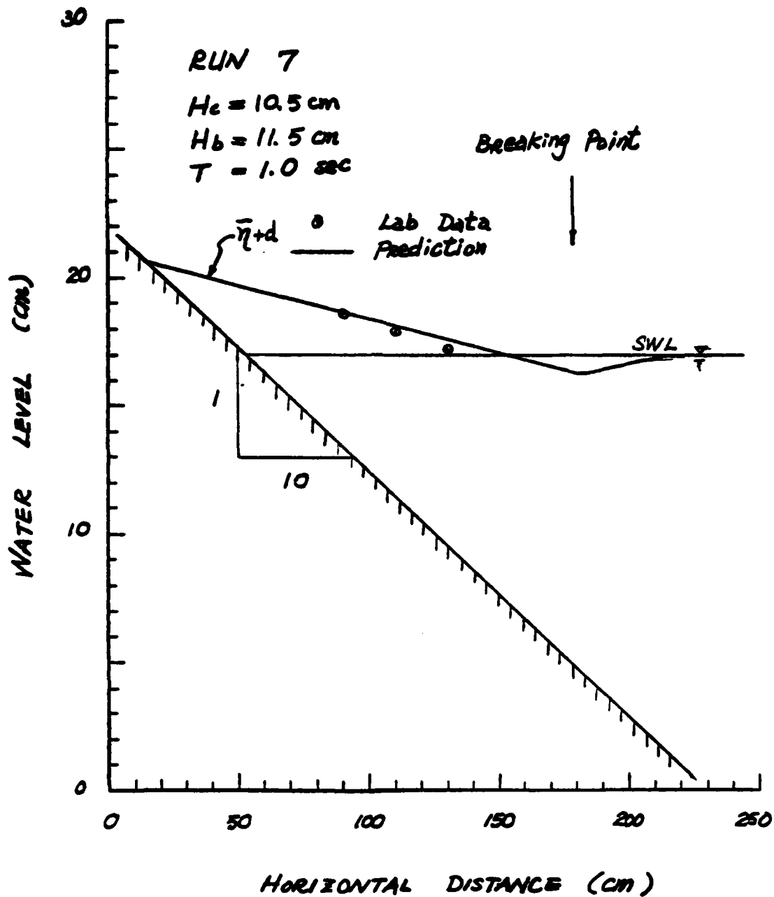
Figure D-4 Wave Run-up Data for Run 7
