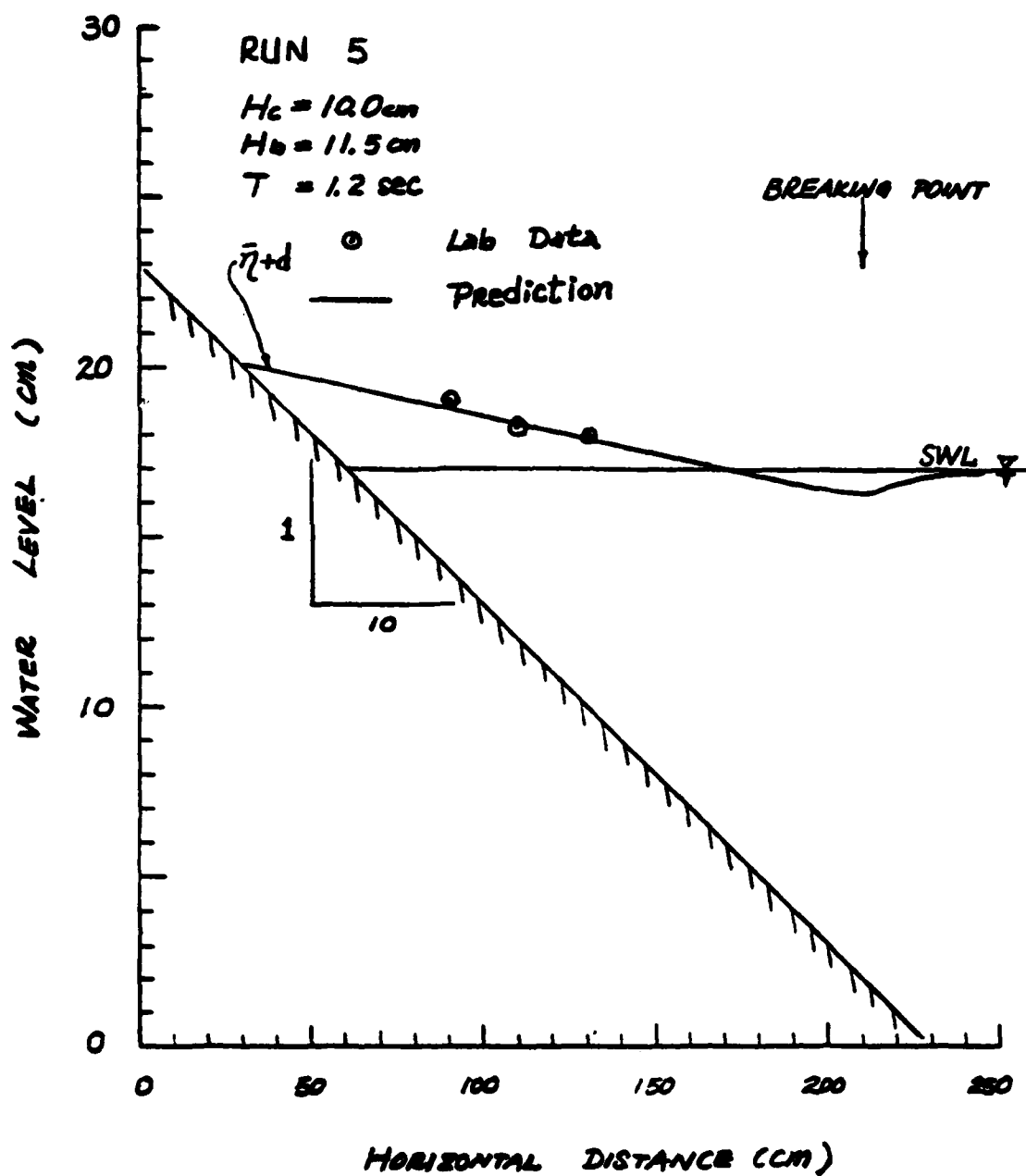
Figure D-2 Wave Run-up Data for Run 5
