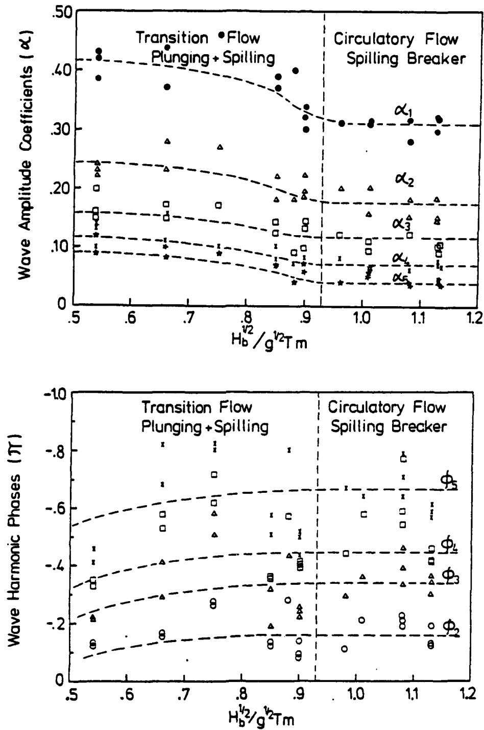
Figure 5-3 Wave Amplitude Coefficients and Phase Coefficients vs. I_w
