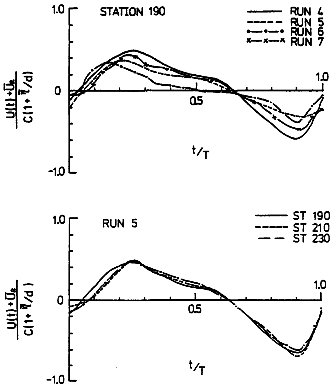
Figure 5-6 Non-dimensional Velocity Profiles
