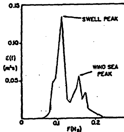
Figure 5.7 Frequency Spectrum Indicating Wind Sea and Swell Peaks (After Long and Hasselmann, 1979)
