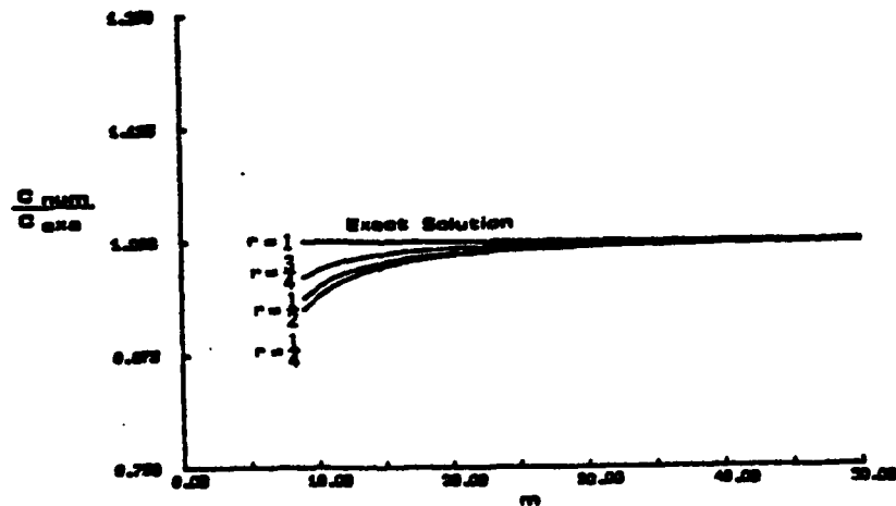
Figure 4.7 Dissipation and Dispersion for the Leap-Frog Scheme
