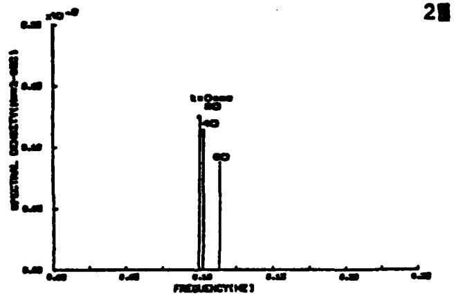
Figure 4.12 Variation of Wave Energy Decreasing with T=10\text{sec} , \theta=20^\circ at Boundary, Location 5III and Location 2III
