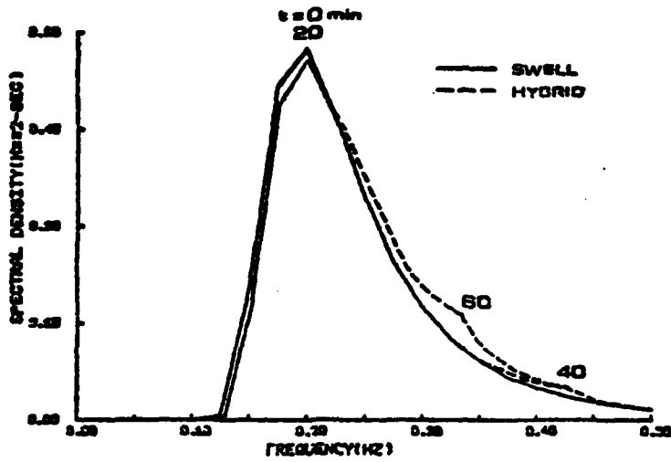
Figure 5.6 Variation of Energy Spectrum due to Decrease of Swell and Increase of Wind Wave at Location 5II and Location 2II
