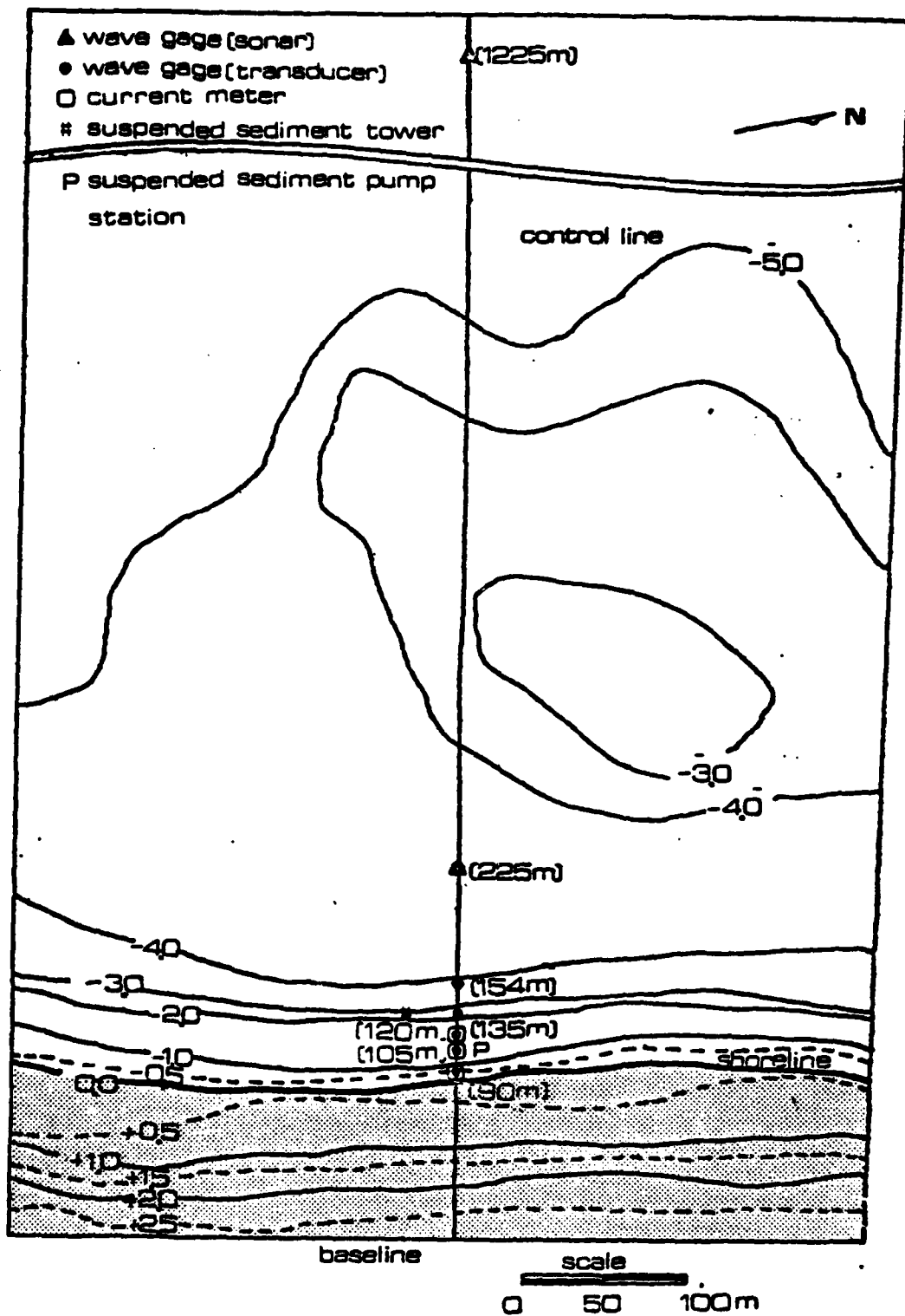
Figure 5.9 Nearshore Field Instrument Arrangement
