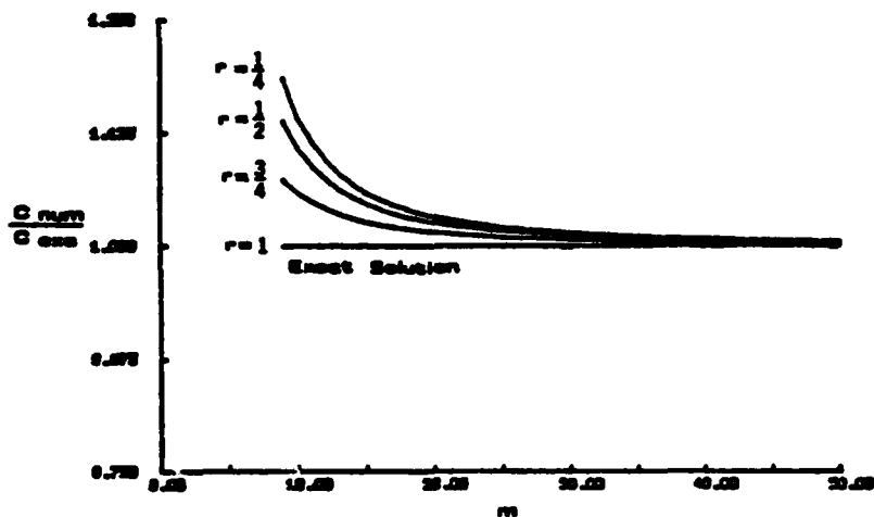
Figure 4.6 Dissipation and Dispersion for the Lax-Friedrichs Scheme
