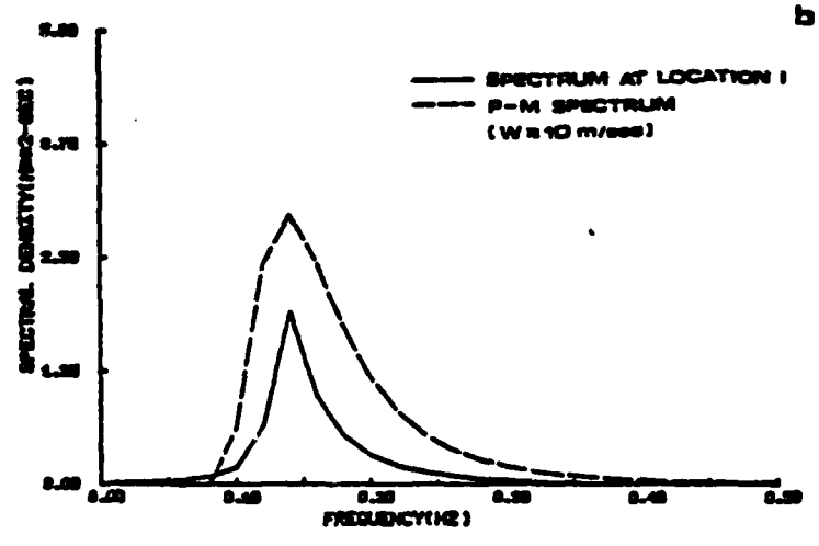
Figure 2.4 Wind Blows over a Deep Uniform Bottom
