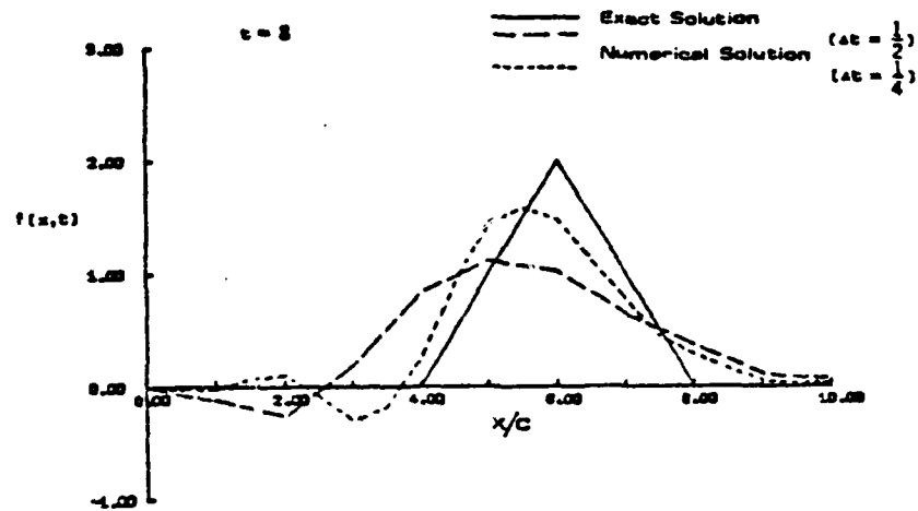
Figure 4.5 Comparison of Exact and Numerical Solutions for r=1/2
