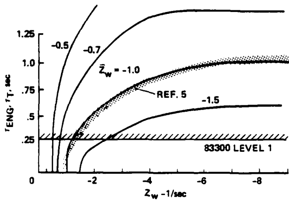
Fig. 14. Trade-off between Z_w and \tau_T for configurations of Fig. 1.
