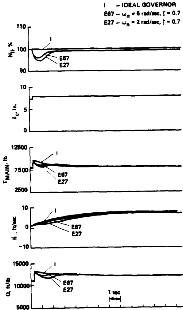
Fig. 8. Engine response time histories; collective steps ( Z_w = -0.65 \text{ sec}^{-1} ).
