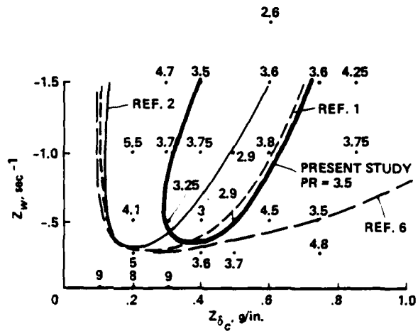
Fig. 11. Vertical damping and collective sensitivity - bob-up maneuver.
