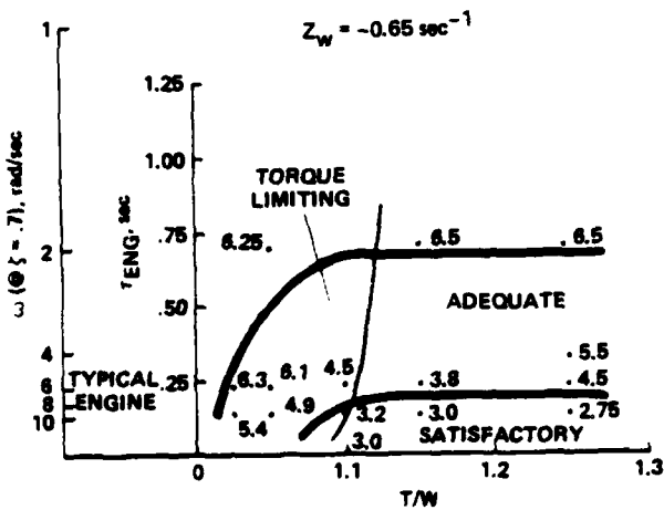
Fig. 9. Engine response time versus T/W - bob-up maneuver.
