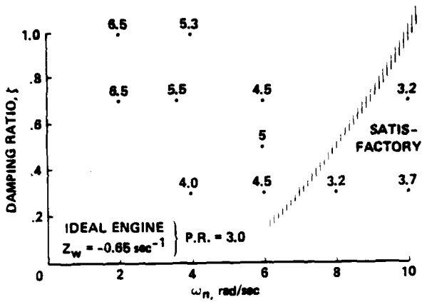
Fig. 7. Effects of engine frequency and damping - quick stop/bob-up.
