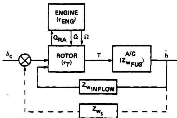
Fig. 2. Helicopter vertical control.
