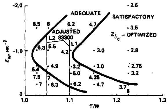
Fig. 13. Vertical damping and T/W - bob-up maneuver.
