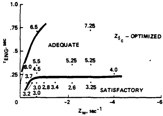
Fig. 15. Trade-off between Z_w and \tau_{eng} for the hover bob-up.
