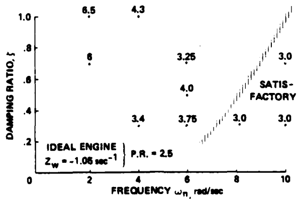
Fig. 6. Effects of engine frequency and damping - dolphin.
