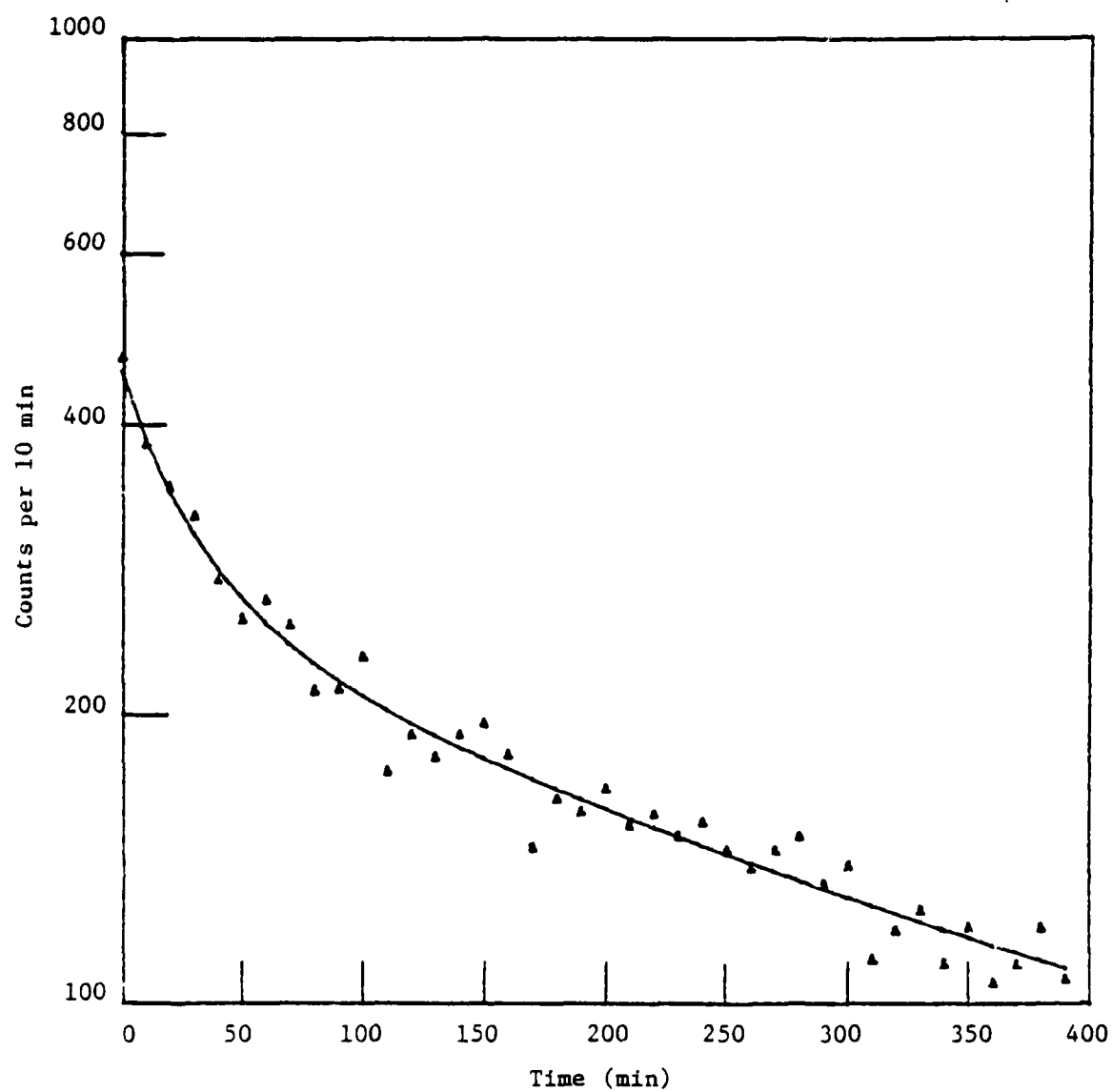
Figure 4.16 Decay curve of stainless activity
