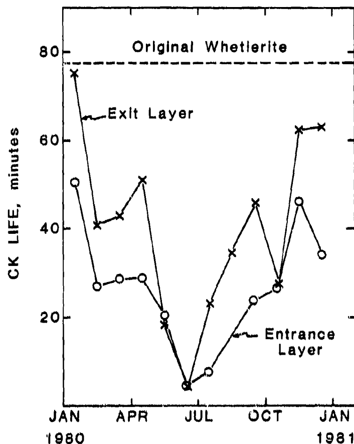
Figure 13. Influence on CK Life after Weathering Whetlerite (2-281) in One-Month Intervals at NRL
