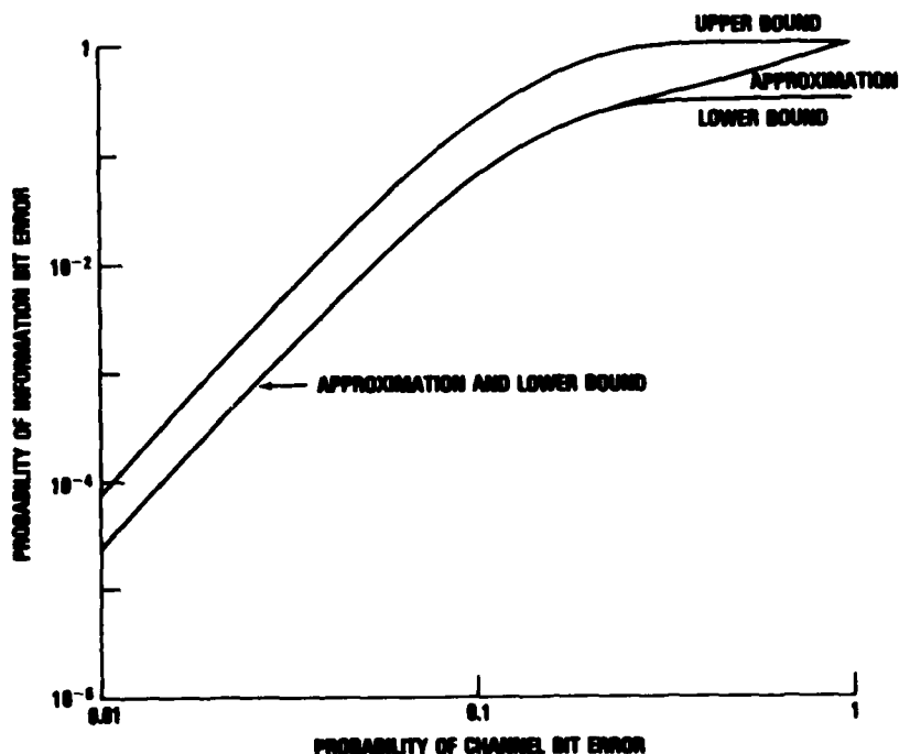
Figure A-1. Information bit error probability as function of channel bit error probability for Golay (23,12) code.
