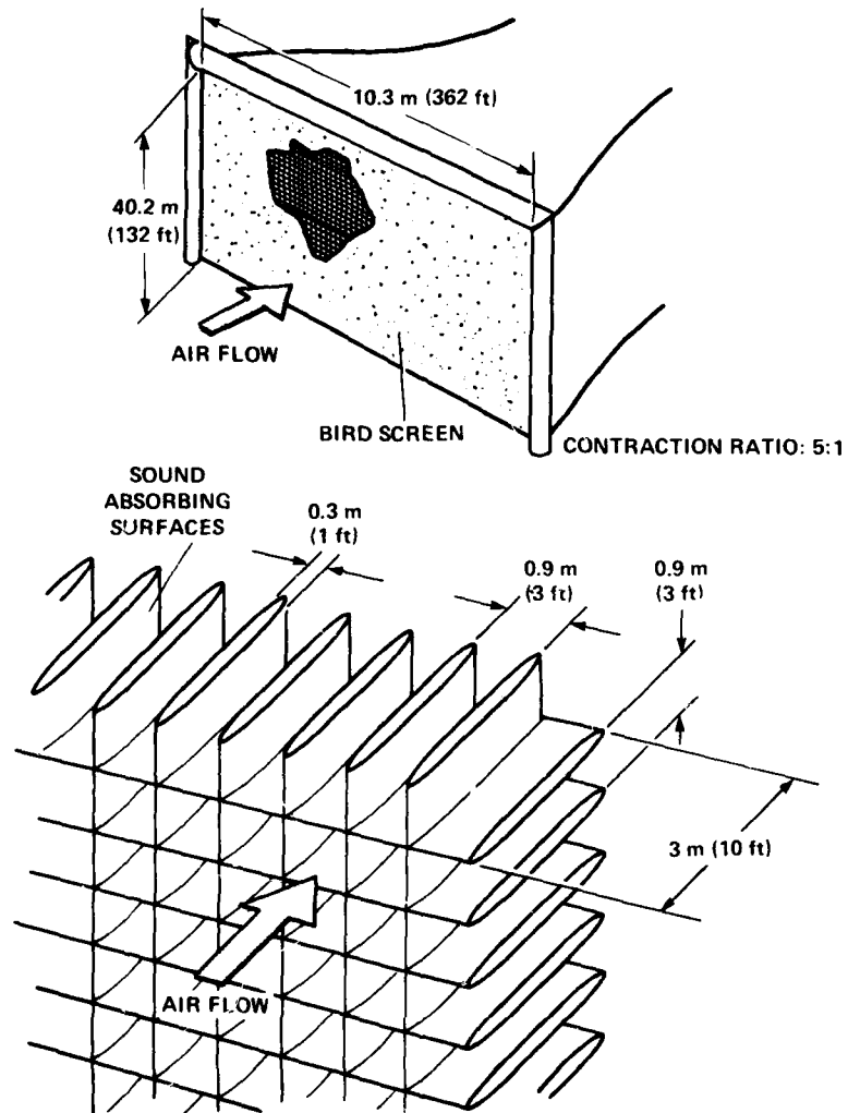
Fig. 6. Inlet flow-straightener and acoustic-baffle system for the selected minimum-protection inlet.
