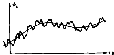
Fig. 3. Typical phase fluctuations: phase jitter and frequency drift.
