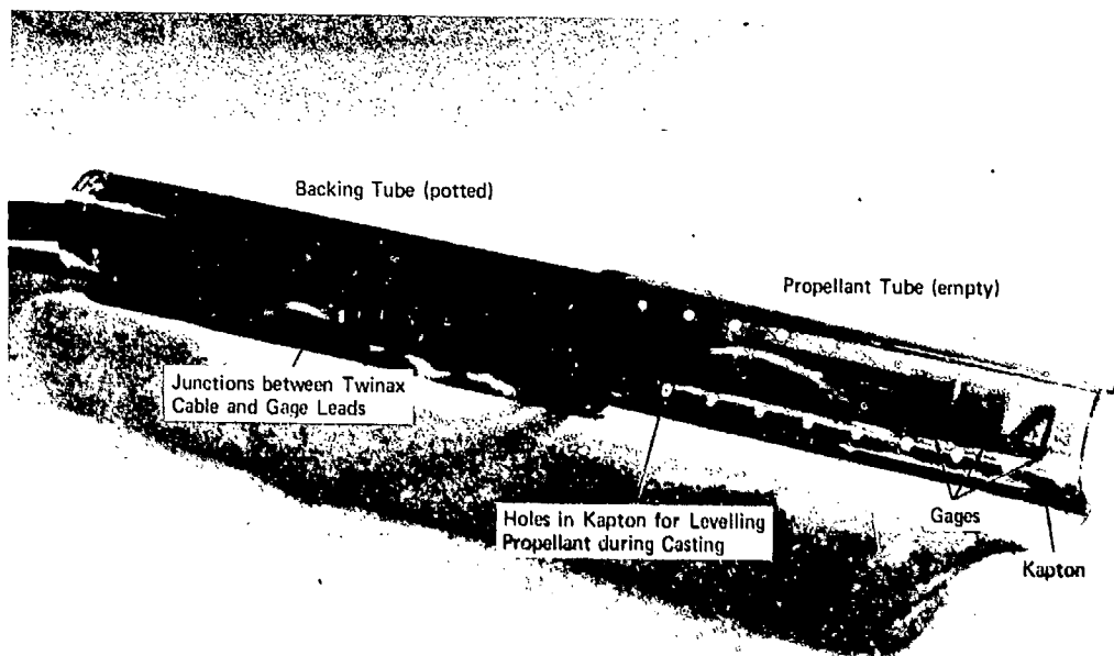
(a) Side View of Kapton Gage Package
