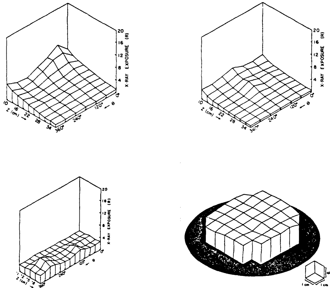
Figure 14. X-ray exposure profiles using no ion source for TLD's in both drift tube wall and endplate configurations.
