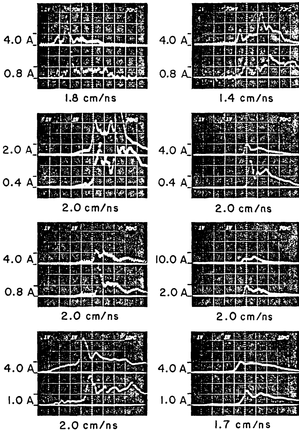
Figure 2. Results for ion time of flight using H ion source. The upper/lower trace is the signal from the Cu mesh/Al plate. The average ion velocity over many shots is 1.8 cm/ns (4 inch I.D. drift tube) and 1.3 cm/ns (9.5 inch I.D. drift tube) where the pulse leading edge is used for measurements.
