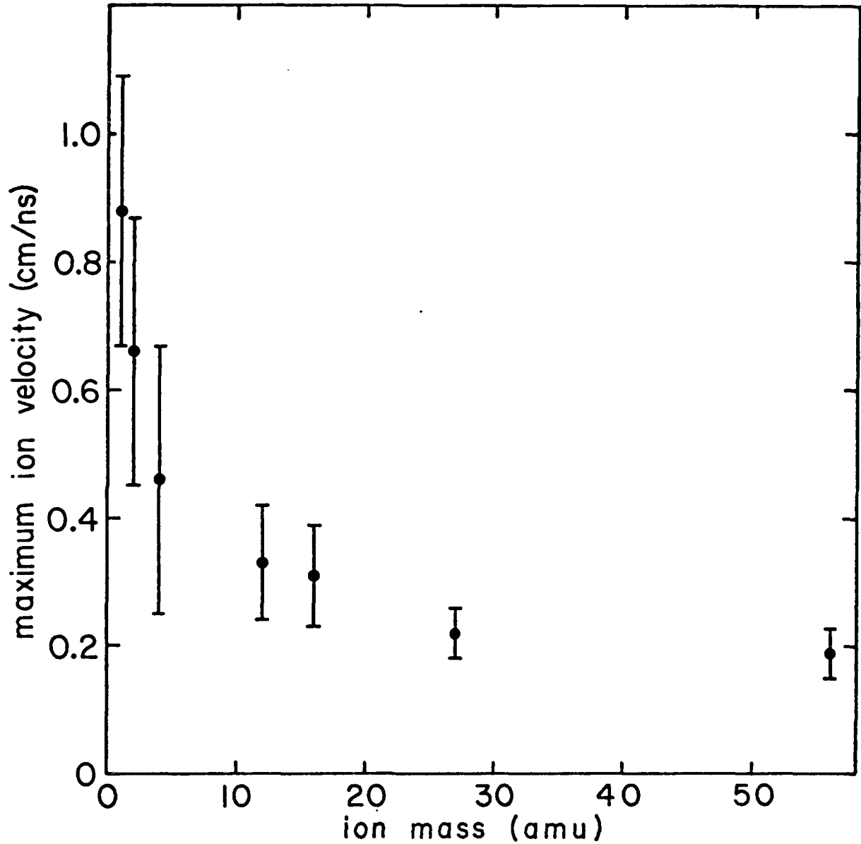
Figure 7. Plot of maximum ion velocity versus ion mass as summarized from the data in Table 2. Note the data for all ions having the same mass, regardless of charge state, are combined (e.g. C^{3+} , C^{2+} , and C^+ ). The error bars represent the standard deviation in maximum ion velocity over several shots.
