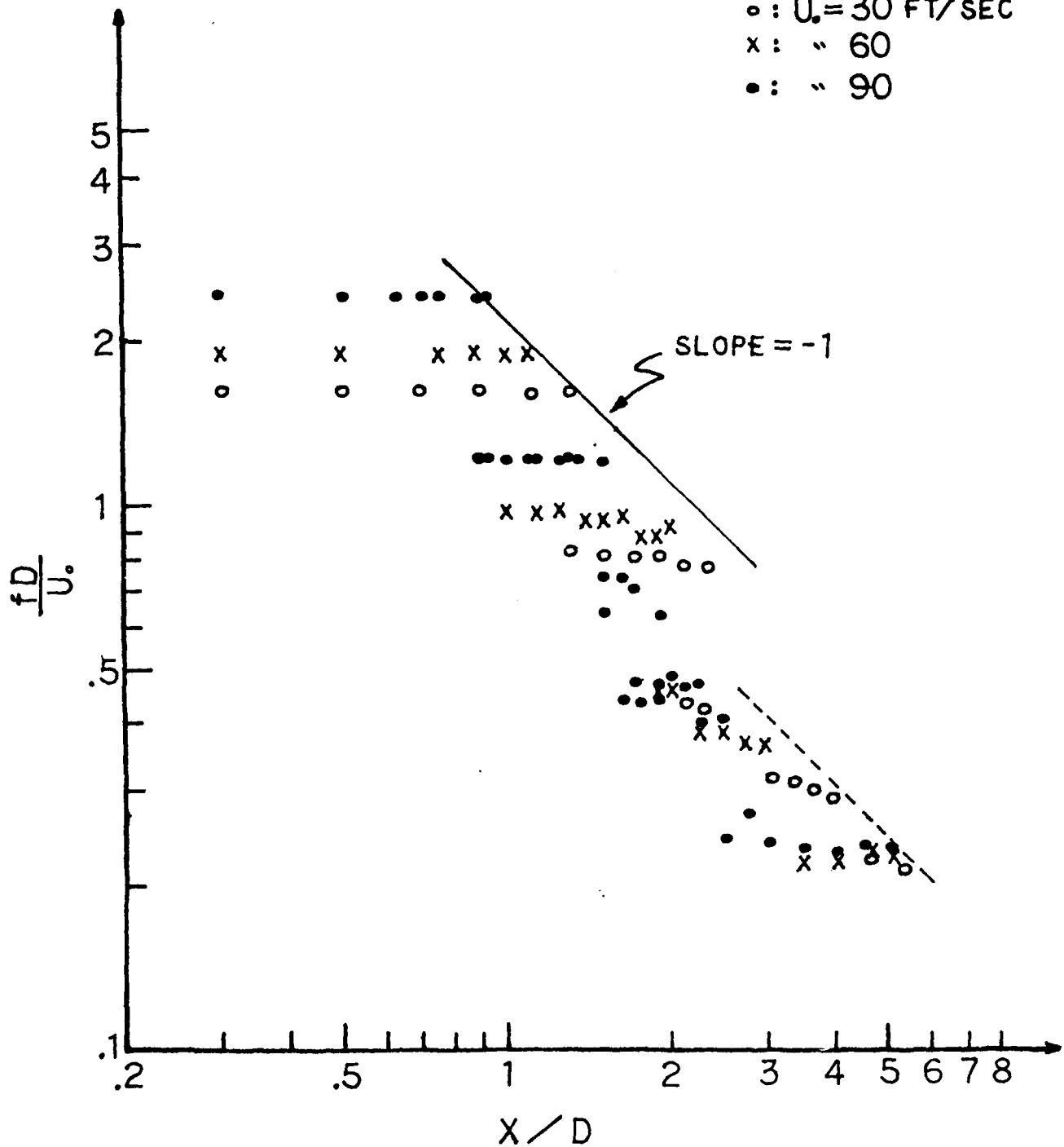
Figure 2. Vortex passage frequency as a function of streamwise distance (free jet).
