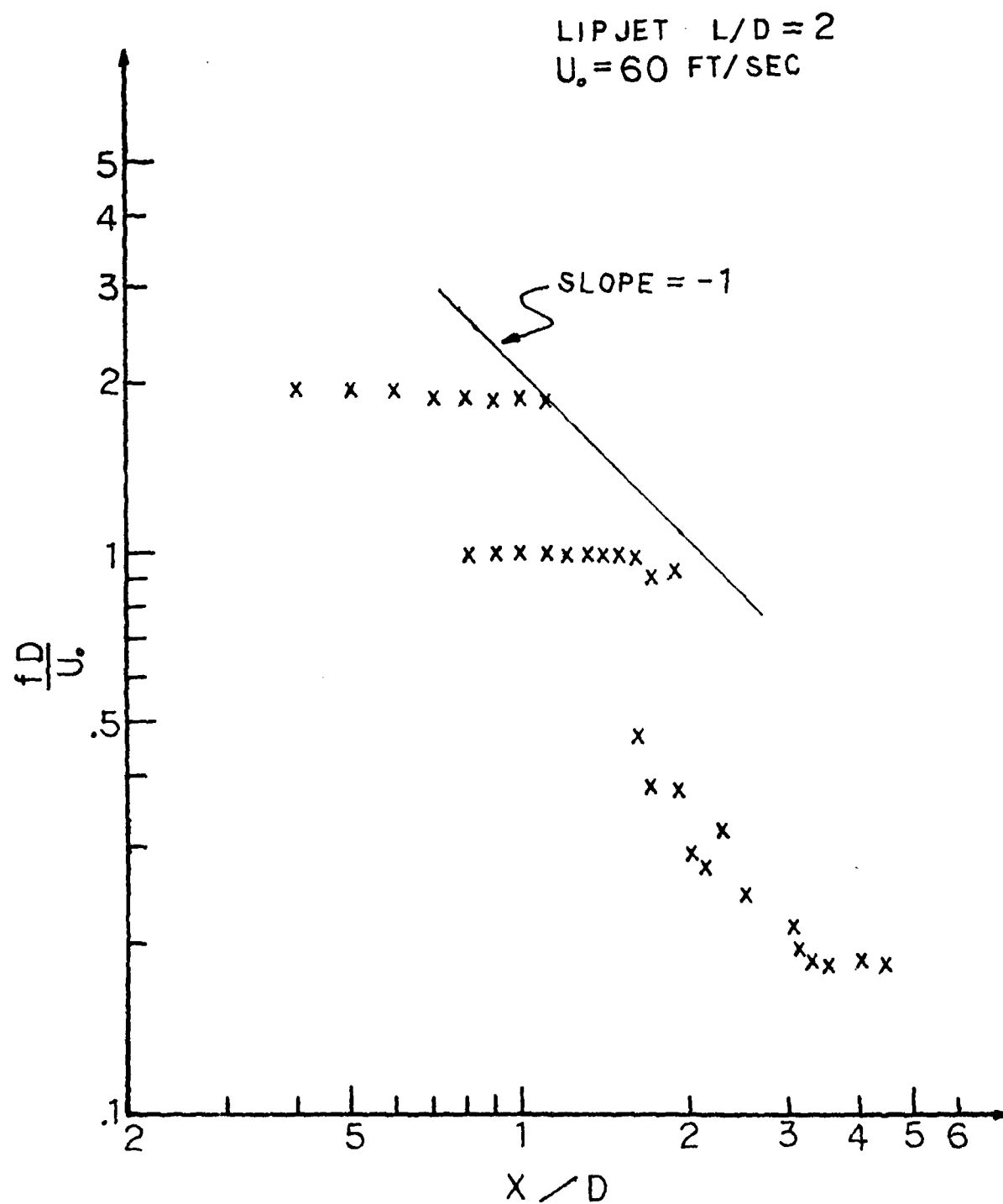
Figure 3. Vortex passage frequency as a function of streamwise distance (lip jet).
