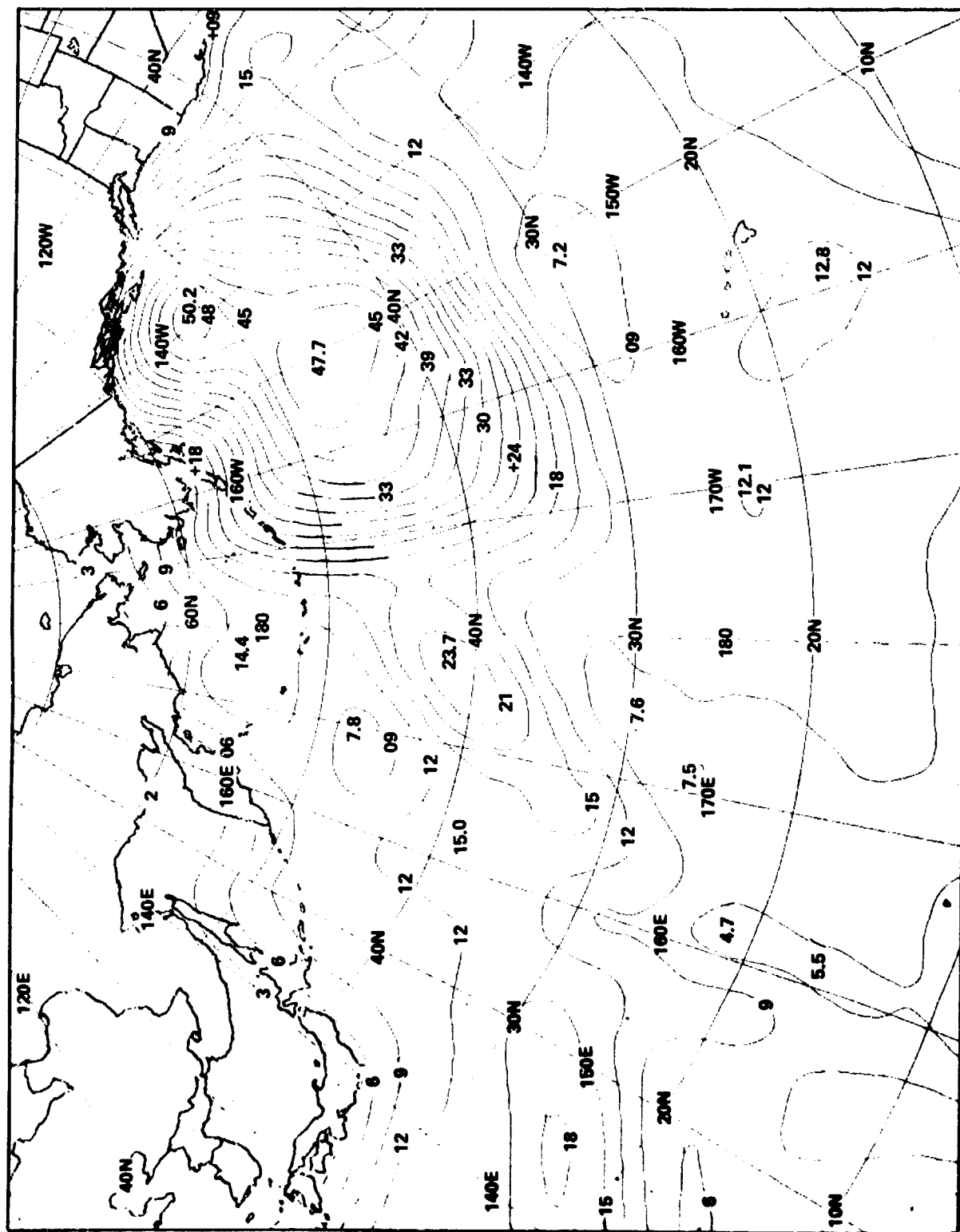
Figure 22 - Significant Wave Height Field (Feet) for 12z 27 October 1977
