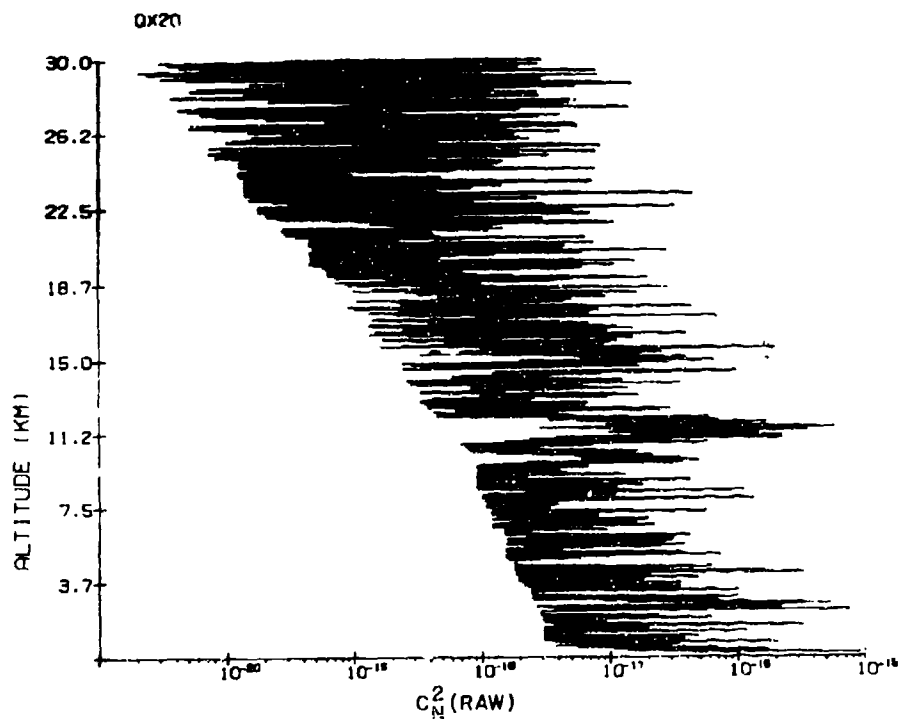
Figure 15. Raw Thermosonde C_N^2 Analysis - Profile Plot. Low and high gain measurements have been combined into a single best measurement. The thermosonde measures C_N^2 from ground level to 30 km. C_N^2 is calculated from C_N^2 and the radiosonde measurements of pressure and temperature
