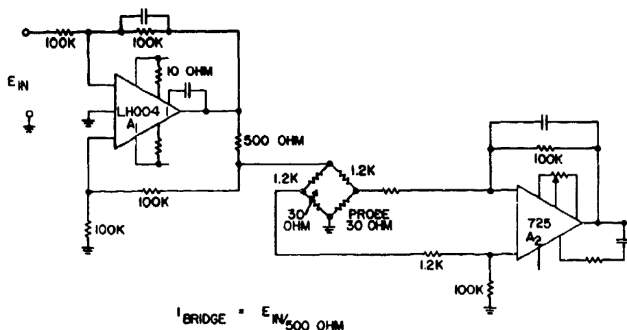
Figure 3. Schematic of Thermosonde Sensor Convective Heat Transfer Test Circuit. For a given input voltage, E_{\text{in}} , the LH0041 circuit produces a constant probe current of (E_{\text{in}} / (2 \times 500)) amps. The 725 amplifier provides an output, E_o = 83.33 \times \text{Bridge potential difference} . Thus the differential resistance of the bridge due to probe I^2R heating is: R = E_o / 83.33 I_i
