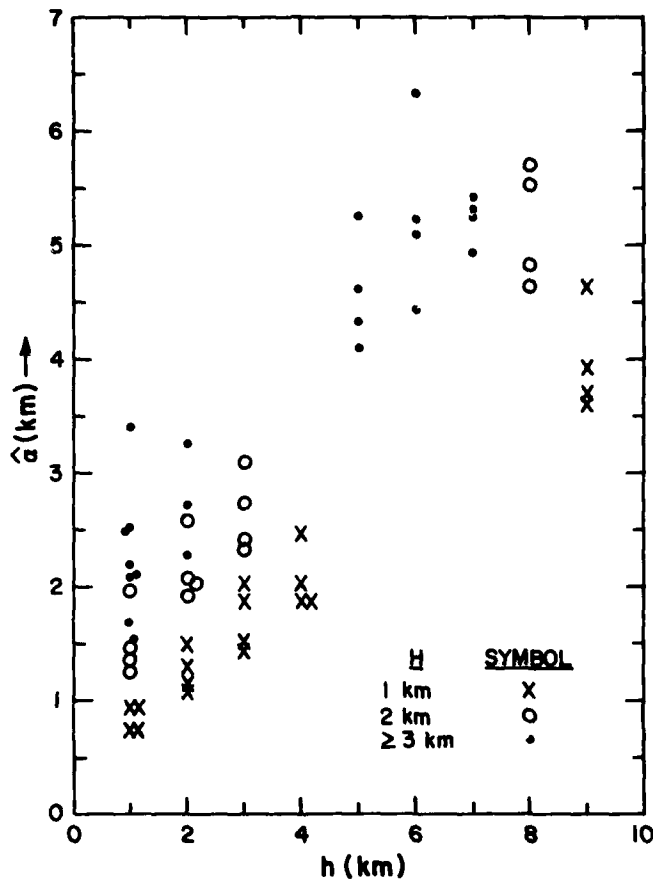
Figure 4. Plot of \hat{\alpha} , Against Thickness (h) of the Atmospheric Layer. The values of \hat{\alpha} are computed from the values of deBary and Moller (1963) for \bar{P}_H , \bar{P}_{H+h} and \bar{P}_h from German flights [Eq. (8)]
