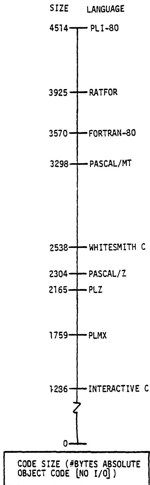
Figure 6-1. Benchmark Results
