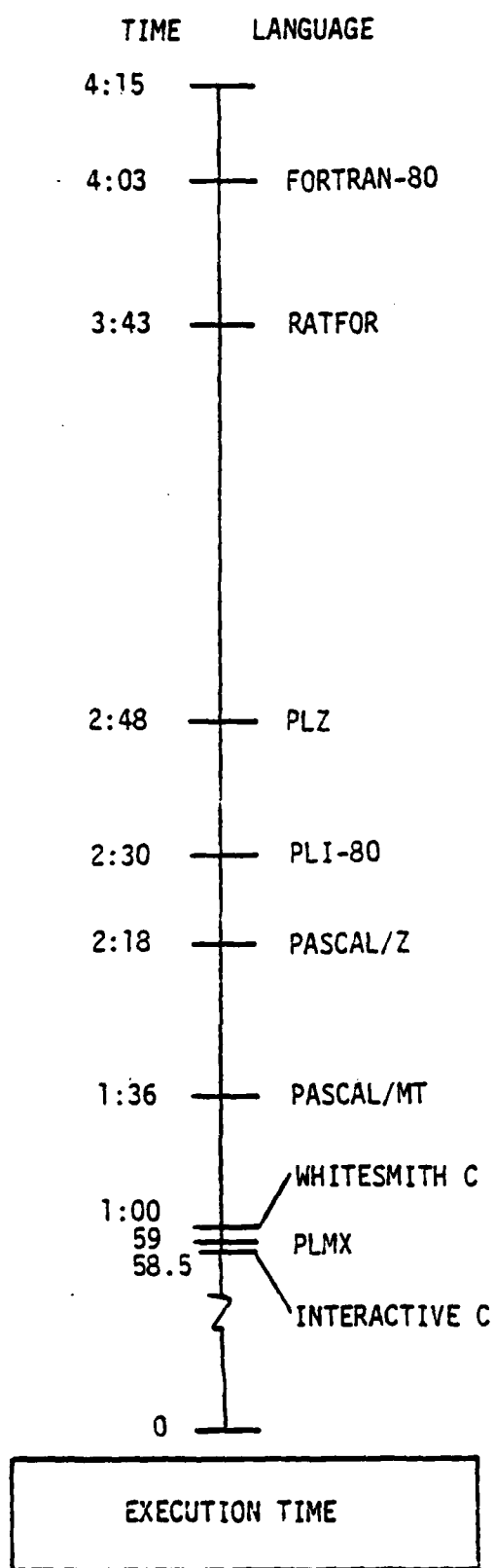
Figure 6-1. Benchmark Results
