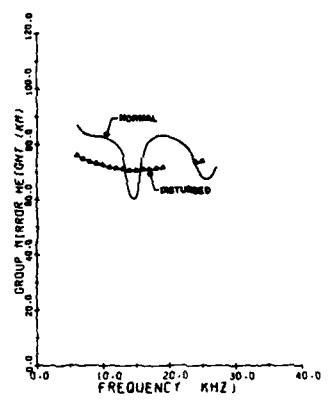
I. GROUP MIRROR REFLECTION HEIGHTS AND ASSOCIATED n_p REFLECTION COEFFICIENTS FROM PERPENDICULAR SKYWAVE DATA
