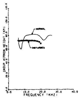
H. GROUP MIRROR REFLECTION HEIGHTS AND ASSOCIATED n_p REFLECTION COEFFICIENTS FROM PARALLEL SKYWAVE DATA
