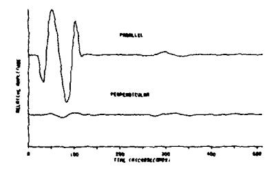
F RECEIVED WAVEFORMS - DISTURBED CONDITIONS 1415 UT 1 AUG 1979 (DOY 213)
