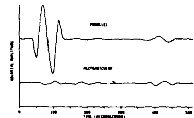
G. RECEIVED WAVIFORMS - NORMAL CONDITIONS 0800 UT 23 APR 1979 (DOY 114)
