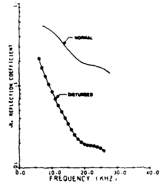
H. GROUP MIRROR REFLECTION HEIGHTS AND ASSOCIATED R_p REFLECTION COEFFICIENTS FROM PARALLEL SKYWAVE DATA
