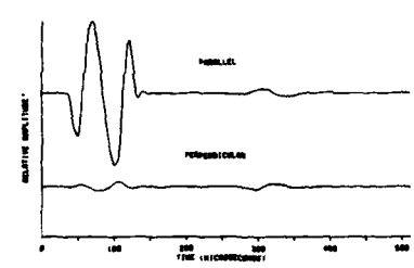
F. RECEIVED WAVIFORMS - DISTURBED CONDITIONS 1700 UT 27 MAY 1979 (DAY 147)
