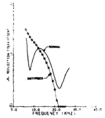
H. GROUP MIRROR REFLECTION HEIGHTS AND ASSOCIATED n_p REFLECTION COEFFICIENTS FROM PARALLEL SKYWAVE DATA
