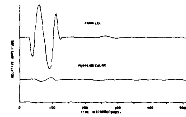
F. RECEIVED WAVEFORMS DISTURBED CONDITIONS (200 UT 3 APR 1979 (DOY 93))
