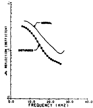
H. GROUP WARROR REFLECTION HEIGHTS AND ASSOCIATED \mu_{\parallel} REFLECTION COEFFICIENTS FROM PARALLEL SKYWAYE DATA
