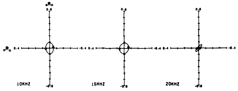
K. SKYWAVE POLARIZATION ELLIPSES - NORMAL CONDITIONS
