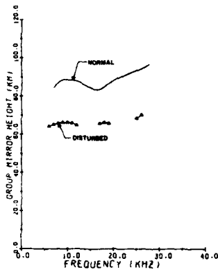
I. GROUP MIRROR REFLECTION HEIGHTS AND ASSOCIATED R_p REFLECTION COEFFICIENTS FROM PERPENDICULAR SKYWAVE DATA
