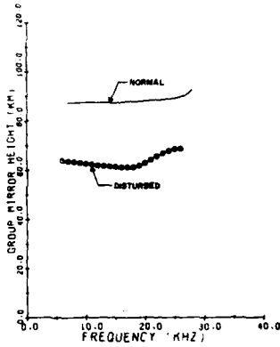
H. GROUP MIRROR REFLECTION HEIGHTS AND ASSOCIATED R_p REFLECTION COEFFICIENTS FROM PARALLEL SKYWAVE DATA
