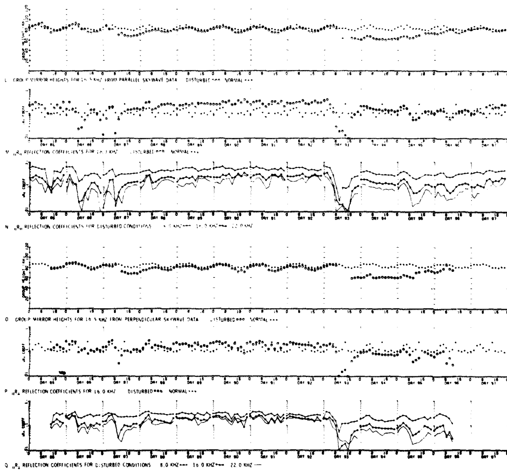
Figure 9. VLF/LF Ionospheric Reflectivity Data for 3 April 1979 (DAY 093) Solar Particle Event (contd)
