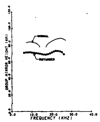
H. GROUP WARDER REFLECTION HEIGHTS AND ASSOCIATED R_p REFLECTION COEFFICIENTS FROM PARALLEL SKYWAY DATA
