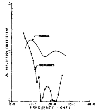
I. GROUP MIRROR REFLECTION HEIGHTS AND ASSOCIATED R_p REFLECTION COEFFICIENTS FROM PERPENDICULAR SKYWAVE DATA
