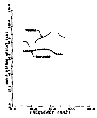
J. GROUP WARDER REFLECTION HEIGHTS AND ASSOCIATED R_p REFLECTION COEFFICIENTS FROM PERPENDICULAR SKYWAY DATA
