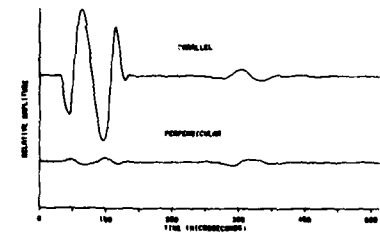
F. RECEIVED WAVIFORMS - DISTURBED CONDITIONS 0800 UT 24 APR 1979 (DOY 114)
