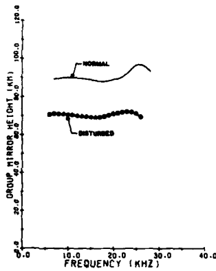
H. GROUP WARROR REFLECTION HEIGHTS AND ASSOCIATED \mu_{\parallel} REFLECTION COEFFICIENTS FROM PARALLEL SKYWAYE DATA
