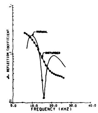
H. GROUP WARDER REFLECTION HEIGHTS AND ASSOCIATED R_p REFLECTION COEFFICIENTS FROM PARALLEL SKYWAY DATA
