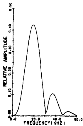
Figure 5. Fourier Amplitude Spectrum of Transmitted Pulses
