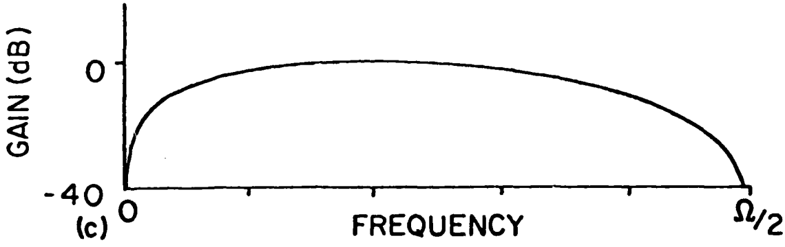
Fig. 7. Behavior of "converged" Howells-Applebaum sidelobe canceller. (a) Antenna pattern plotted at jammer frequency. (b) Frequency response in jammer direction. (c) Frequency response in signal direction.
