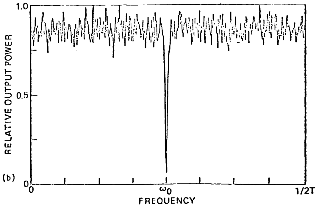
Fig. 5. Results of two-weight adaptive noise cancelling experiments. (a) Primary input composed of cosine wave at 512 discrete frequencies. (b) Primary input composed of uncorrelated samples of white noise.
