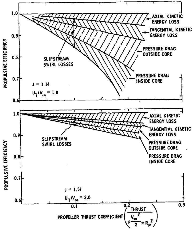
Figure 3. Energy Losses With Slipstream Swirl as a Function of Advance Ratio and Propeller Thrust Coefficient
