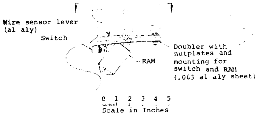
Figure 8. Main rotor actuated cutter.
