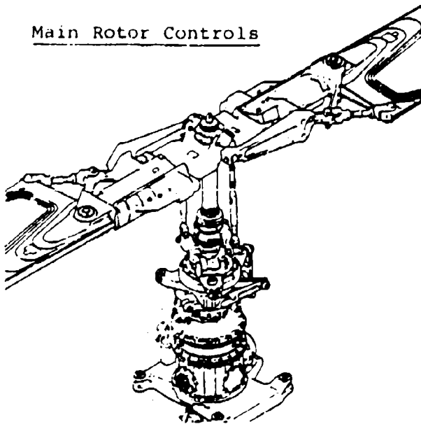
Figure 4. AH-1 helicopter.
