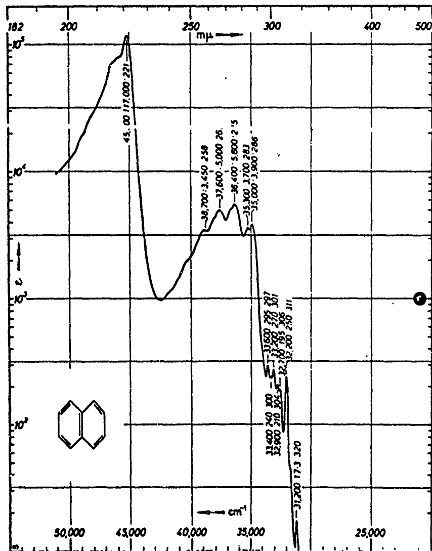
Figure 9. UV Spectrum of Naphthalene in Hexane (From UV Atlas of Organic Compounds, Plenum Press, N.Y.)
