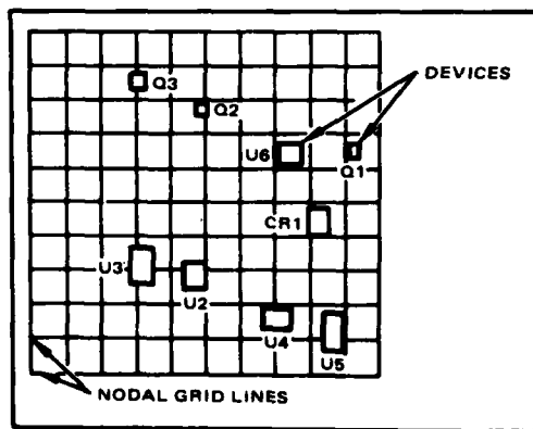
Figure 8-5. This plan view shows a detailed thermal model of a hybrid microcircuit with device locations.
