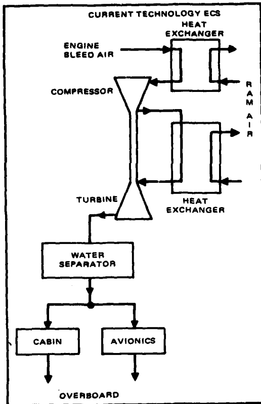
Figure 7-16. Air-cycle refrigeration is used for aircraft ECS.
