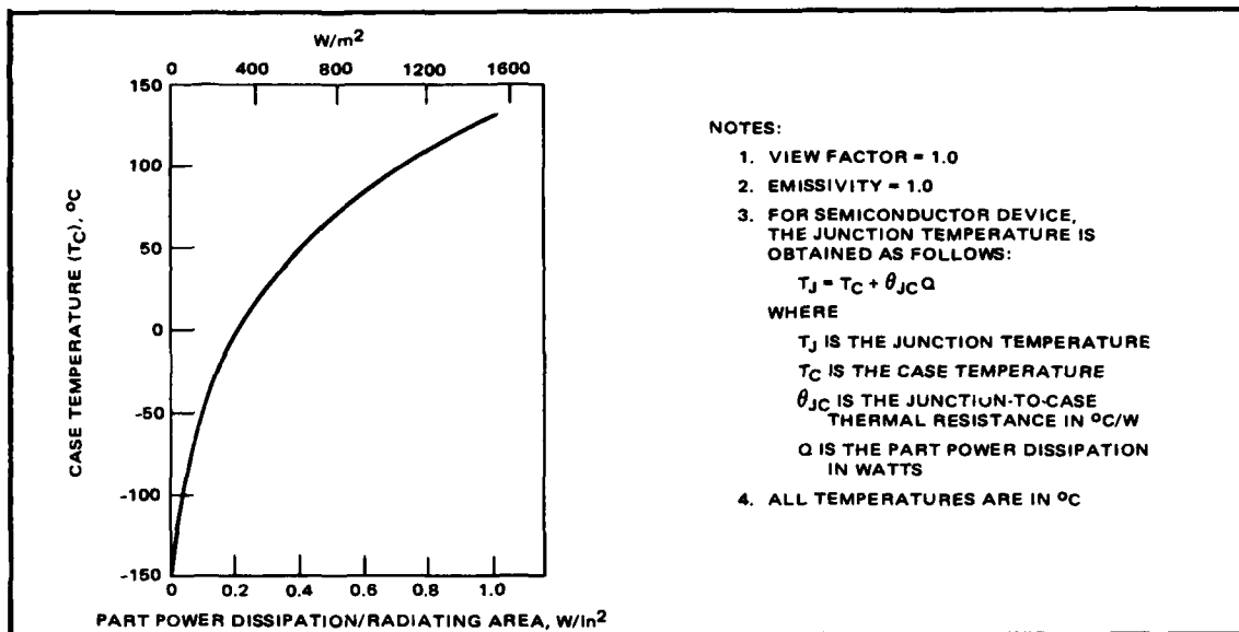
Figure E-11. Estimated temperatures of parts cooled by direct radiation to deep space (Cooling Type K).
