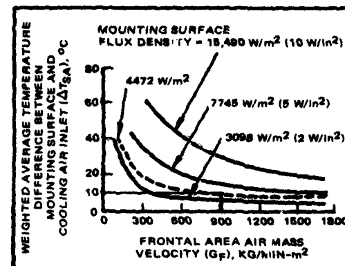
Figure E-6. Estimated temperatures of cold-plate-mounted parts using forced-air cooling (Cooling Type F).
