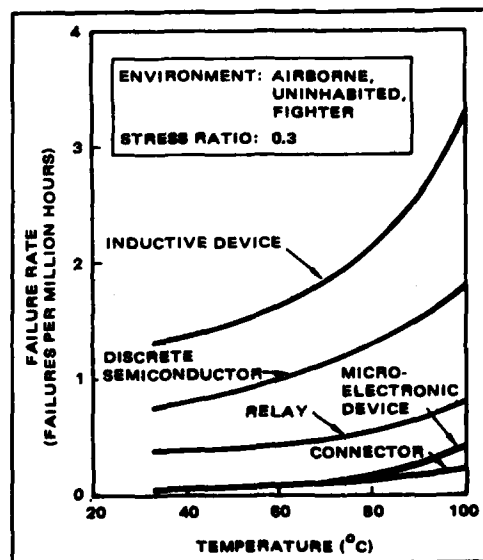
Figure 4-1. Failure rates are accelerated by high temperatures.
