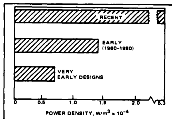
Figure 7-19. A trend in avionic design is the tendency to increase the power density.
