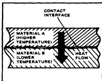
Figure 5-4. An interface between contacting surfaces is a relatively inefficient heat-flow path.
