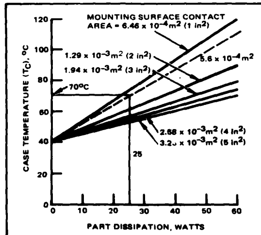
Figure E-12. Estimated temperatures of parts cooled by liquid-transport loop using deep space as the ultimate sink (Cooling Type L).
