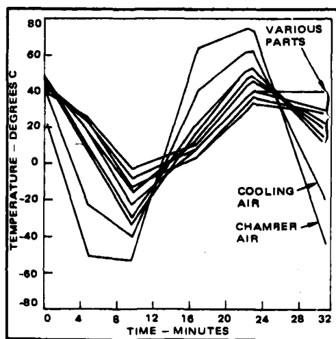
Figure 10-1. Part temperatures lag chamber air temperature.
