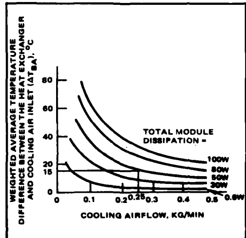
Figure E-5. Estimated temperatures of card-mounted parts using forced-air-cooled flow-through modules (Cooling Type E).
