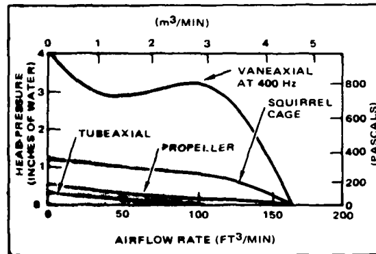
Figure 7-15. Pressure/airflow characteristics are an important consideration in selecting a blower for a specific application.
