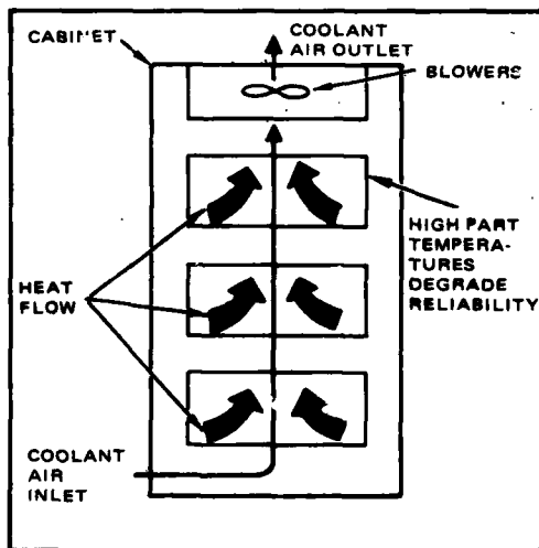
Figure 1-3. In the first redesign, a blower drew coolant air through units serially; but high part temperatures in downstream unit reduced reliability.
