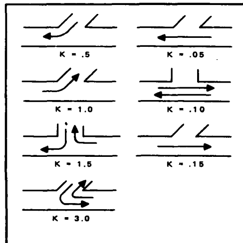
Figure C-1. Turning loss coefficients for fluids.
