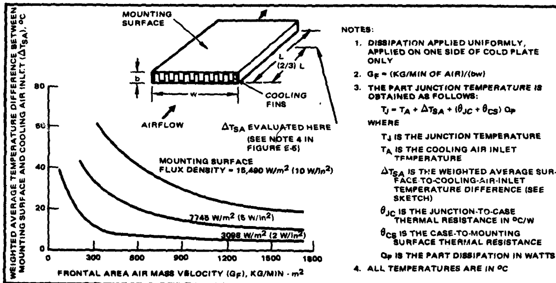
Figure E-6. Estimated temperatures of cold-plate-mounted parts using forced-air cooling (Cooling Type F).
