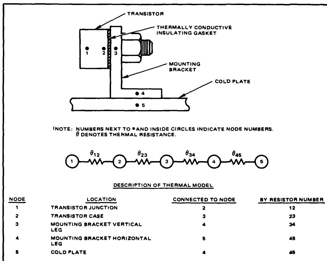
Figure 8-3. A simple thermal model is employed to analyze a transistor, mounting bracket and cold plate assembly.
