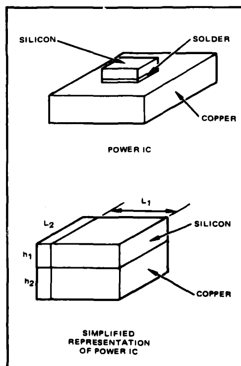
Figure 8-2. An analytical solution can be obtained by a simplified representation. 8-11
