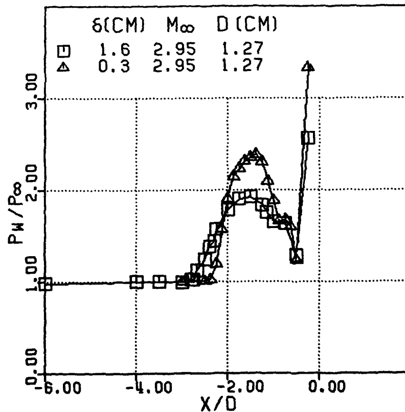
Figure 14. Effects of Boundary Layer Thickness on Mean and R.M.S. Pressure Distributions on Centerline.
