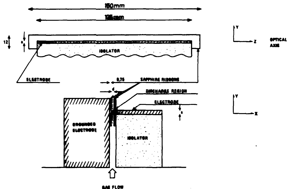
Figure 4.1 The discharge geometry
