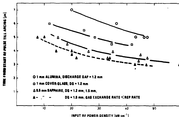
Figure 6.5 Time from start of input rf-pulse till development of large number of arcs, for various dielectric ribbons on the electrodes
