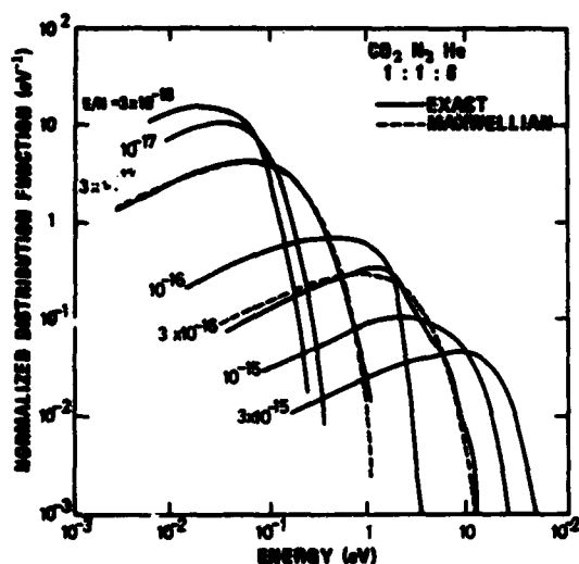
Figure 3.8 Derived electron distribution functions in the gas mixture \text{CO}_2:\text{N}_2:\text{He} = 1:1:8 , for various values of E/N ( \text{Vcm}^2 )
