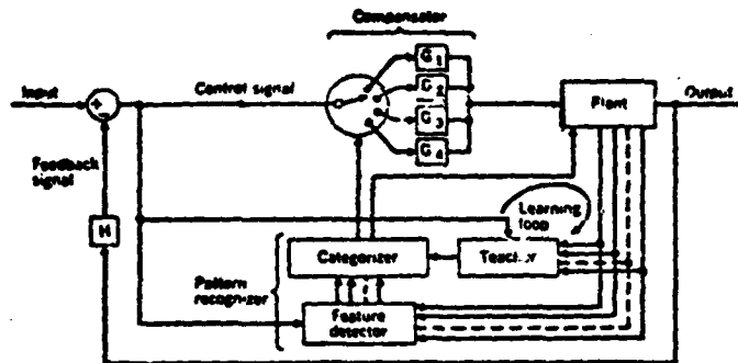
Figure 2 General form of learning control system.
