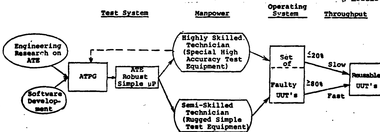
Fig. 1 Overview of System Configuration
