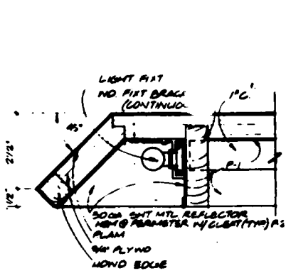
LIGHT FIXT. DETAIL (8) SCALE: 1/2" = 1'
