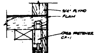
CASE FASTENER CF-1 (12) NO SCALE
