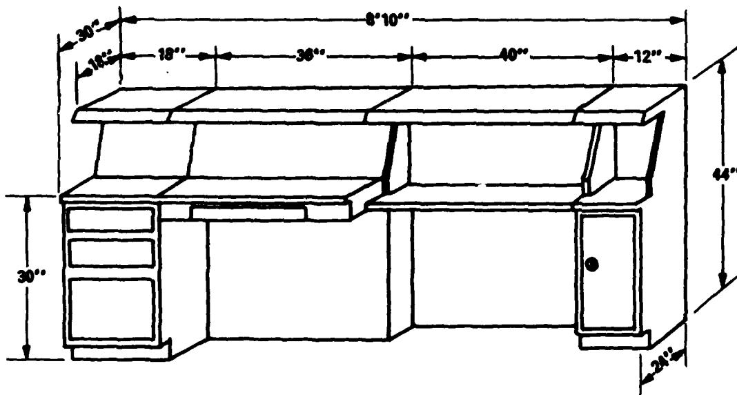
FIGURE 19. SUPERVISOR DESK IN-LINE CONFIGURATION
