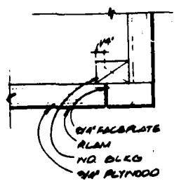
FRONT PNL. DETAIL (12) SCALE: 1/2" = 1'
