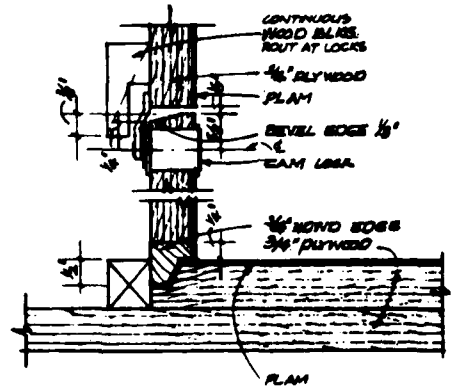
FRONT PNL. DETAIL (11) NO SCALE
