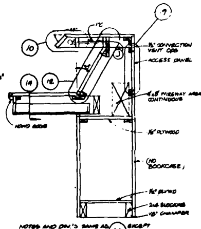
SECTION (9A) (ALT. NO. 1 MAIN CONSOLE)
