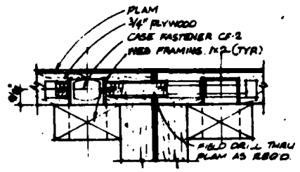
CASE FASTENER CF-2 (10) NO SCALE
