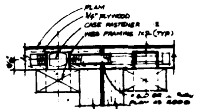
CASE FASTENER CF-2 (16) NO SCALE
