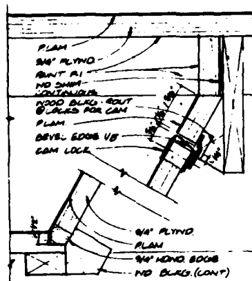
FRONT PNL. DETAIL (9) SCALE: 1/8" = 1"
