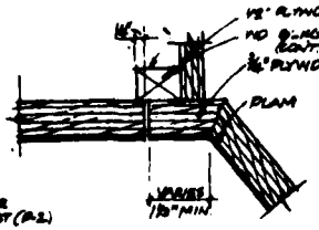
FRONT PNL. DETAIL (15) SCALE: 1/8" = 1"
