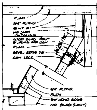
FRONT PNL. DETAIL (9) SCALE: 1/2" = 1'
