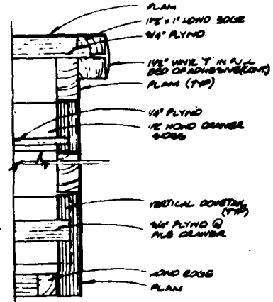
DRAWER DETAIL (11) SCALE: 1/8" = 1"
