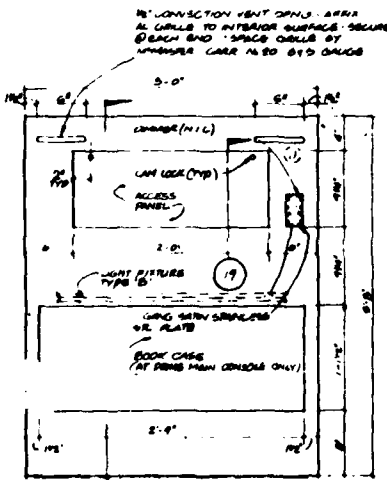
REAR ELEVATION (7A)
