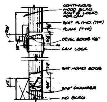
ACCESS PNL. DETAIL (13) NO SCALE
