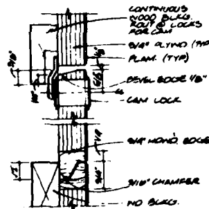
ACCESS PNL. DETAIL (13) NO SCALE
