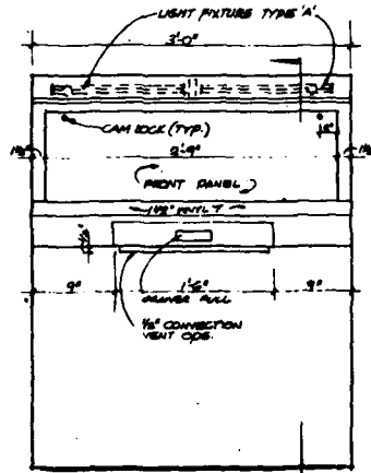
FRONT ELEVATION (8A) (ALT. NO. 1 MAIN CONSOLE)
