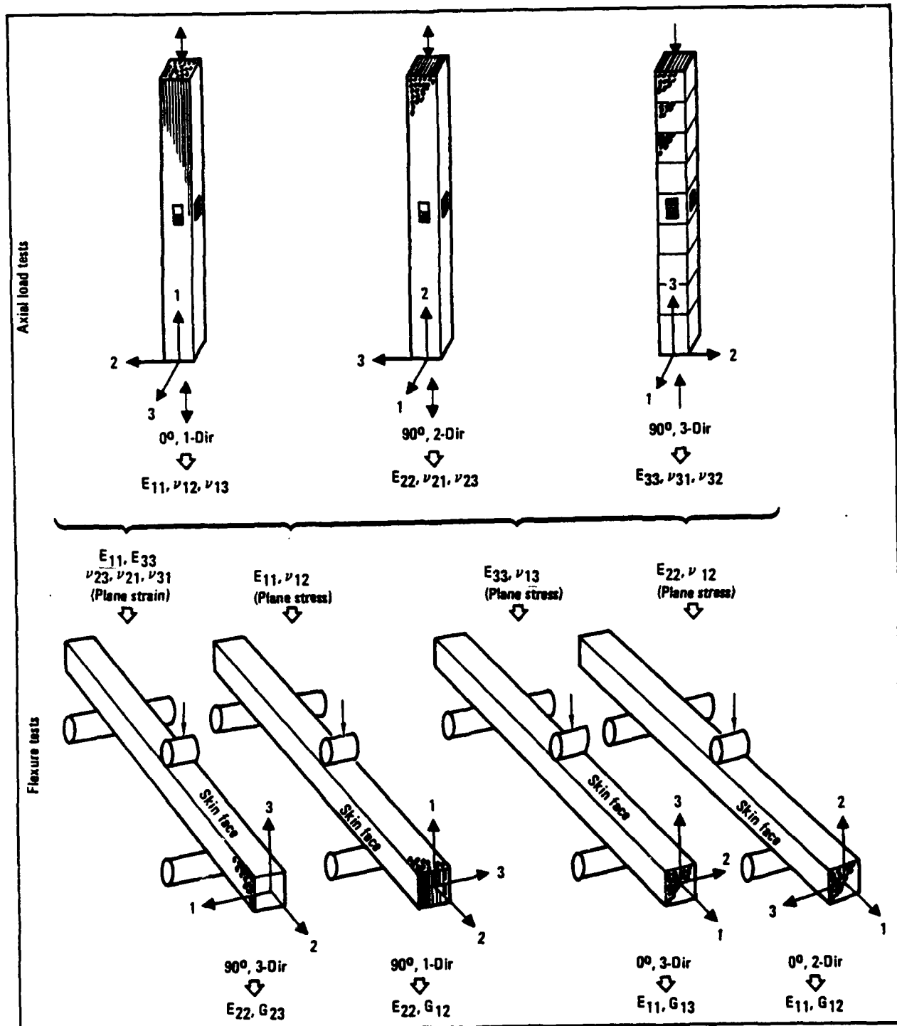
Figure 1. - Test Plan Schematic
