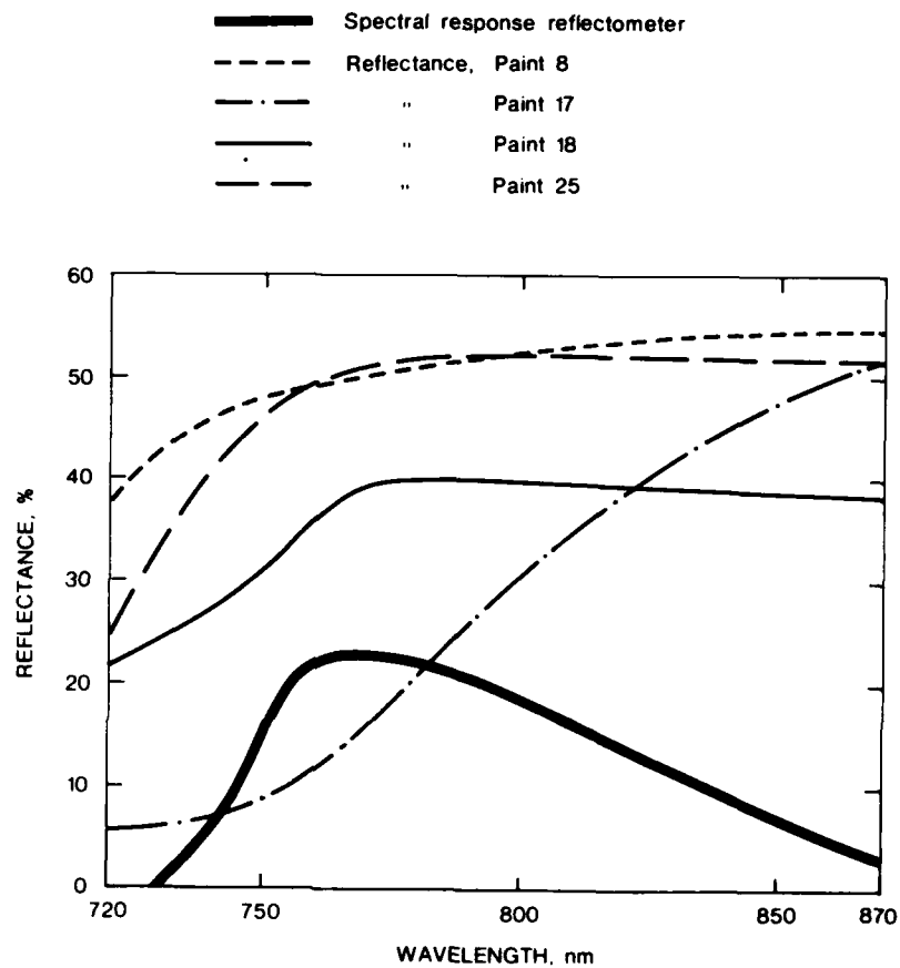
FIG. 4 Reflectance of Paints over the Wavelength Range 720 to 870 nm Compared to the Calculated Spectral Response of the Prototype Reflectometer
