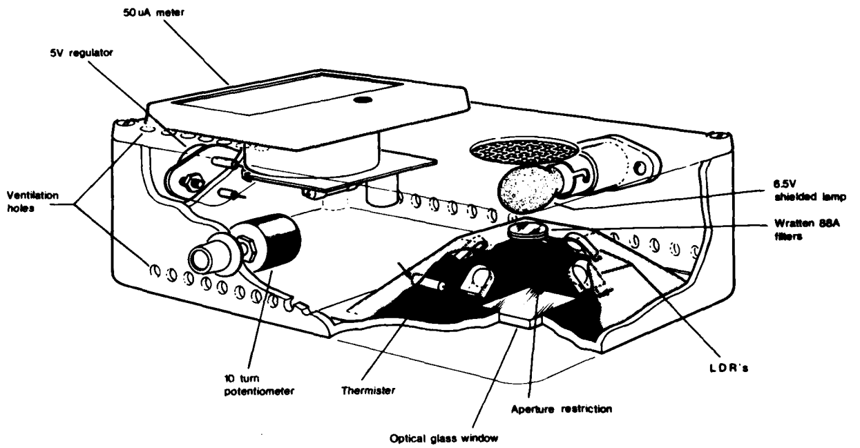
FIG. 1 Diagramatic Representation of Prototype Reflectometer
