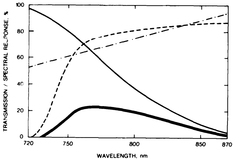
FIG. 3 Variation in Transmission, Emission and Response with Wavelength for Wratten 88A Filter, Tungsten Filament at 2000°C and Elcoma Type LDR and these combined to give the calculated spectral response of the prototype reflectometer
