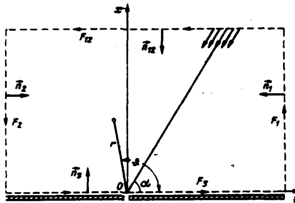
Fig. 5.1. On calculation of radiation pattern of slot in impedance plane.
