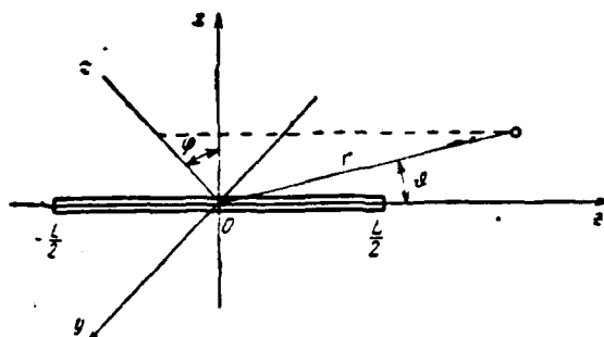
Fig. 2.1. Line-source antenna. Coordinate system.
