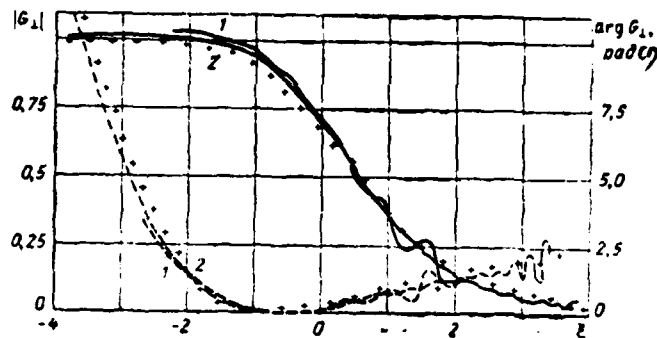
Fig. 6.5. Dependence |G_{\perp}(z)| (solid lines) and \arg G_{\perp}(z) (dotted lines): 1) ka=6 ; 2) ka=30 . Crosses designated asymptotic values |G_{\perp}(z)| and \arg G_{\perp}(z) .
