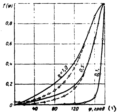
Fig. 5.10. To evaluation/estimate of the accuracy of the approximation/approach of Kirchoff small circles showed approximate values.
