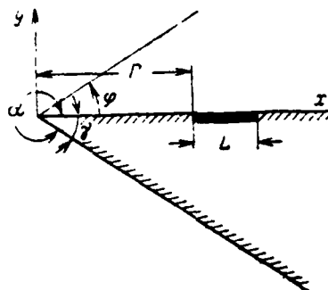
Fig. 4.1. On the calculation of surface antenna, which is located on the key.
