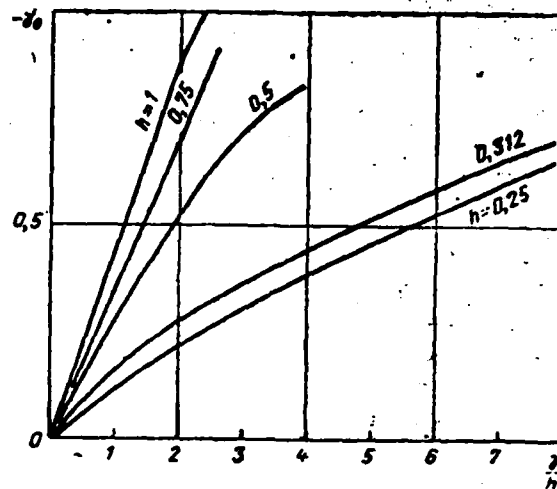
Fig. 8.6. Graph/diagrams of dependence of position of effective phase center on ratio \gamma/h during perpendicular polarization.
