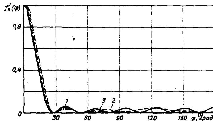
Fig. 6.15. To the evaluation/estimate of the discontinuous distributions of field on the cylinder during the parallel polarization: 1 - radiation pattern f'_n(\varphi) ; 2 - the diagram of six slots, arranged/located with 0 \leq \varphi \leq \pi/2 , 3 - "ideal" radiation pattern.
