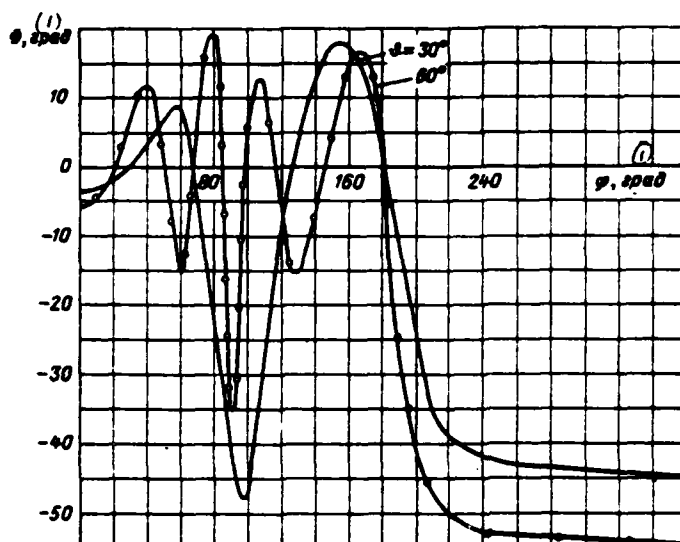
Fig. 9.9. Phase diagrams \Phi_{\phi_1}(\varphi, \theta) = \Phi_{\varphi}(\varphi, \theta) = \arg E_{\varphi}(\theta, \varphi) \Phi_{\varphi}(\varphi, \theta) = \arg E_{\varphi}(\varphi, \theta) .
