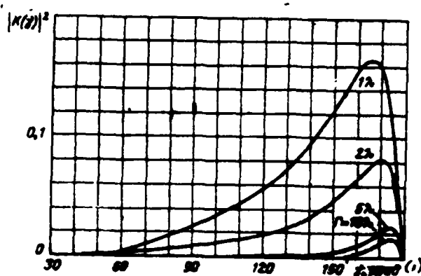
Fig. 4.13. Function |K(\gamma, \alpha F)|^2 with different ones \gamma and r .
