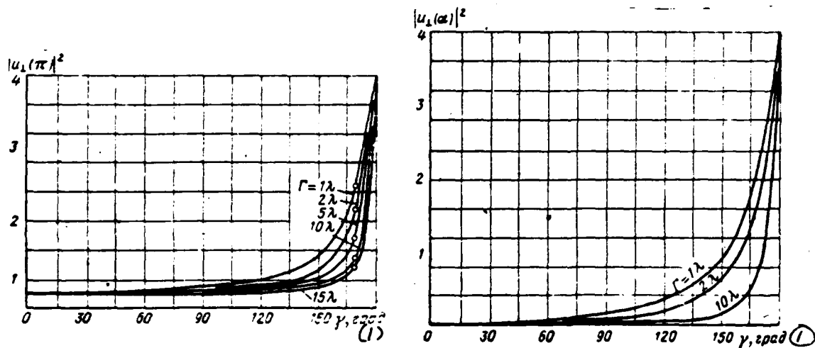
Fig. 4.12. Values |u_\perp(\pi)|^2 and |u_\perp(\alpha)|^2 with different ones \gamma and \Gamma .
