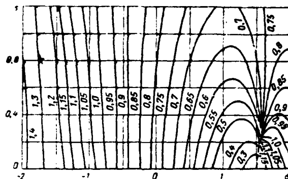
Fig. 3.9. Lines of constant value t_n on the plane \sigma, s , ( \xi=0 ).
