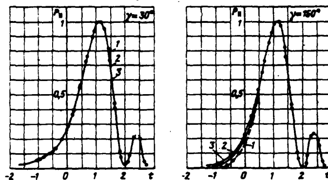
Fig. 4.2. Radiation patterns P_{||}(t) at wedge angle of \gamma=30^\circ and 150^\circ : 1) l=2 ; 2) l=5 ; 3) l=10 .
