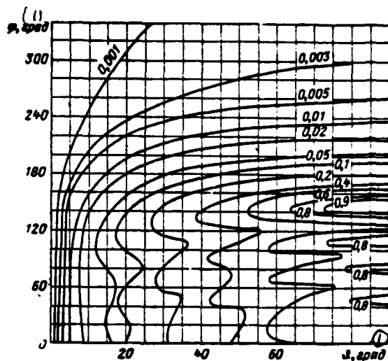
Fig. 9.2. Lines of level |E_{\parallel}(\theta, \varphi)|^2 = \text{const} of the radiation pattern of the longitudinal slot. This diagram is calibrated to its own maximum, and remaining (Fig. 9.3-9.6) to maximums |V(\theta, \varphi)|^2 .
