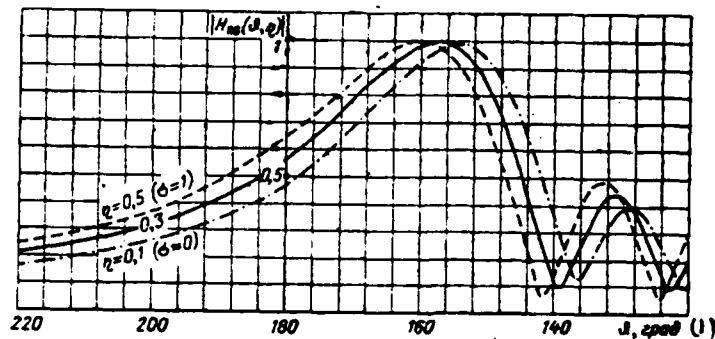
Fig. 5.6. Standardized/normalized radiation patterns of ground waves |H_{\text{gr}}(\theta, \eta)| for the case \gamma=5 and different values \eta .
