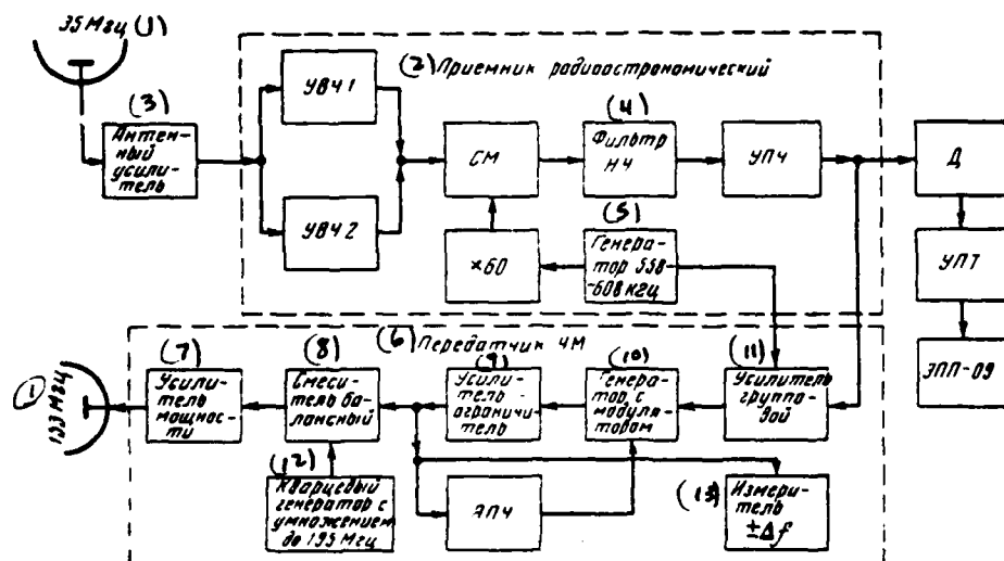
Fig. 1. Block diagram of equipment of extension point/item.
