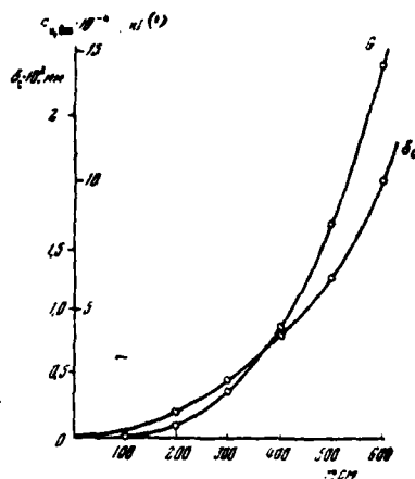
Fig. 5. Graph/diagrams of dependence of maximum sagging/deflection on rim of bushing \delta_c and weight of bushing G_{н.в.т} on radius r .
