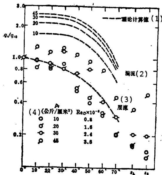
Fig. 2 Heat Flux Distribution Along Surface for Smooth Wall Model With d=0
