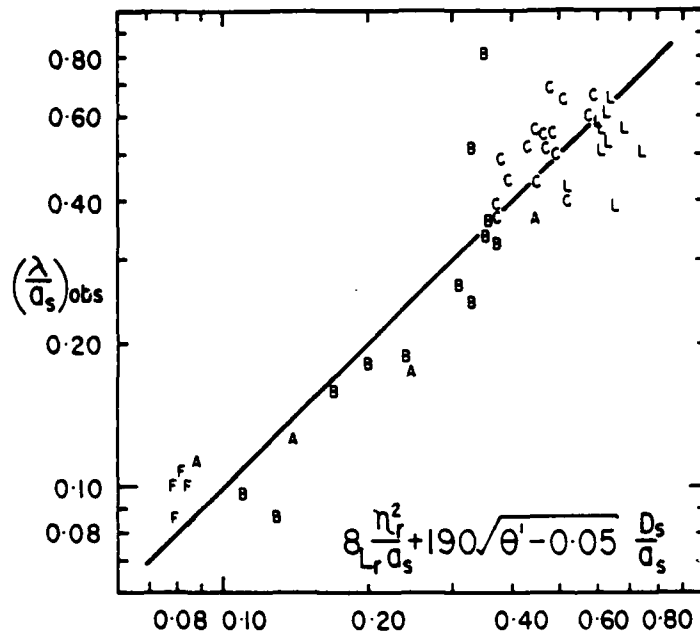
Figure B7: Comparison between predicted and measured roughness to semi excursion ratios.
