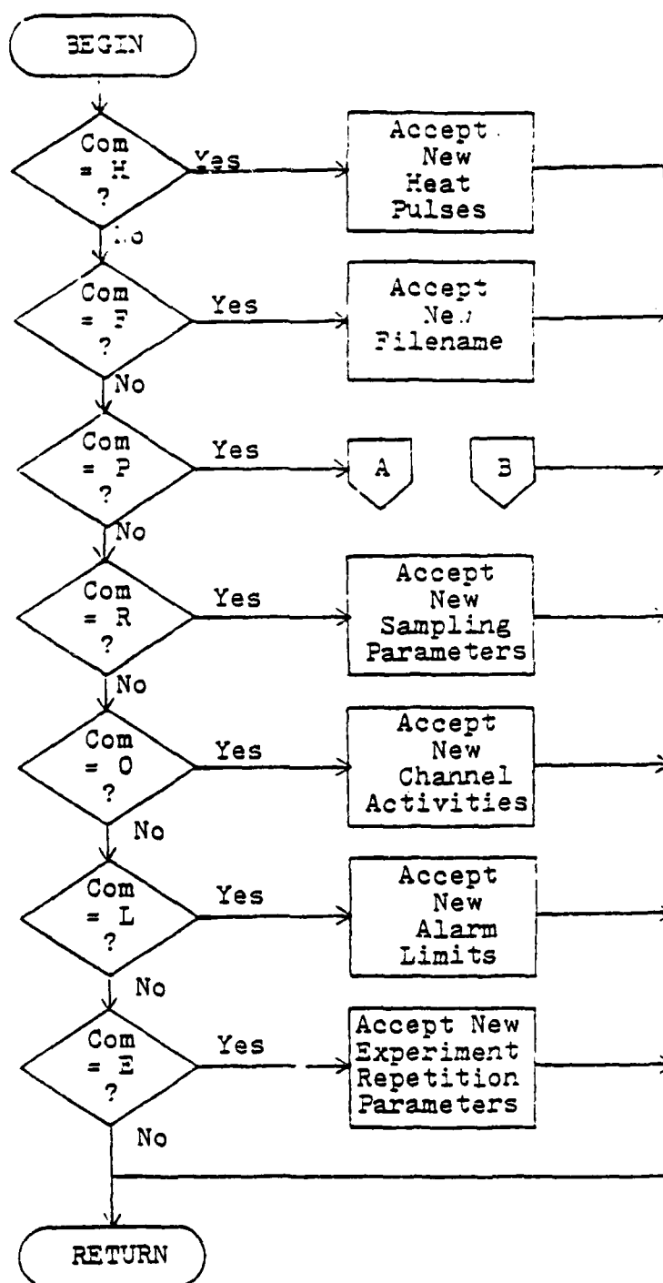
Figure 16. Flowchart of Subroutine UPDATE
