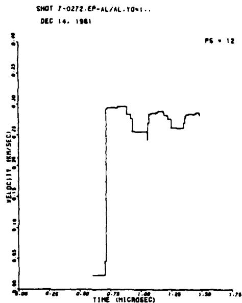
Figure 4. Free Surface History Calculated by SWAP for Shot 272. \gamma = 1 kbar, \sigma_s = 12 kbar.
