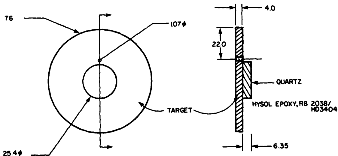
Figure 6. Target Design Using Fused Silica Window. (Dimensions in mm.)
