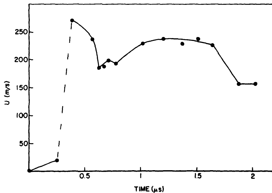
Figure 5. Measured Free Surface Velocity for Shot 272.
