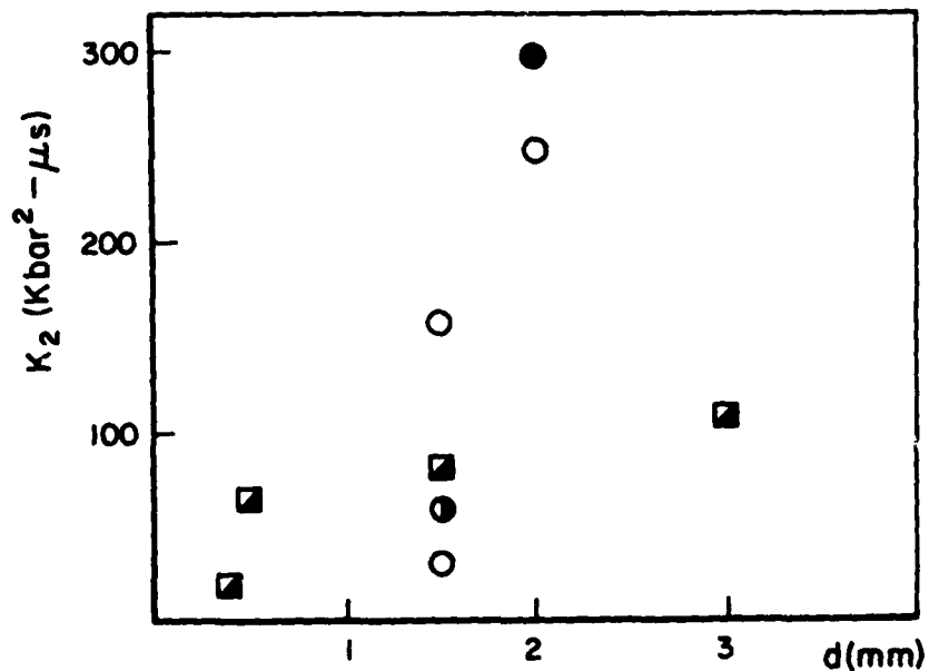
Figure 14. Damage Parameter K_2 for Spall in OFHC Copper. (Squares are data from reference 10.)
