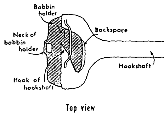
Figure 28. Nomenclature for parts of the bobbin mechanism.
