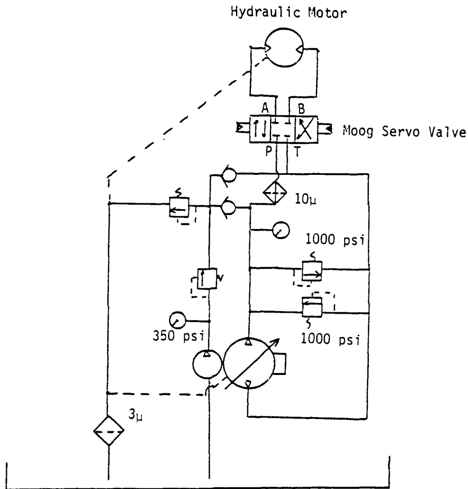
FIGURE 5. Hydraulic Circuit of Demonstration Unit
