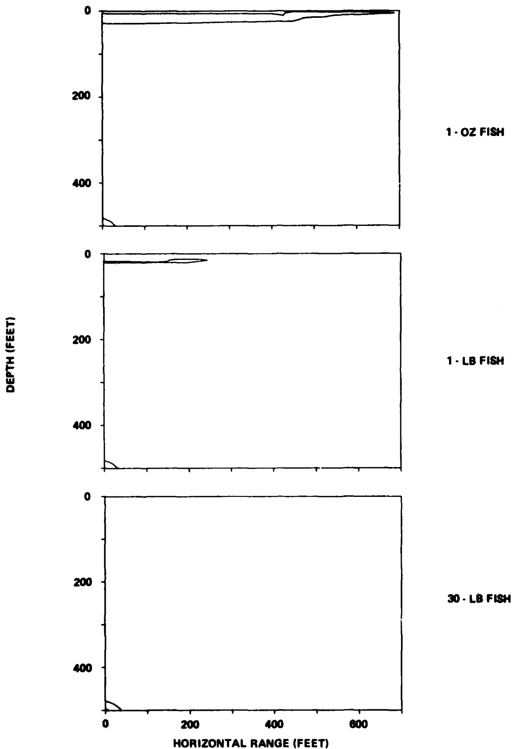
FIGURE 3-2 10% KILL PROBABILITY CONTOURS FOR WELLHEAD SEVERANCE EXPLOSION - 500-FT WATER DEPTH
