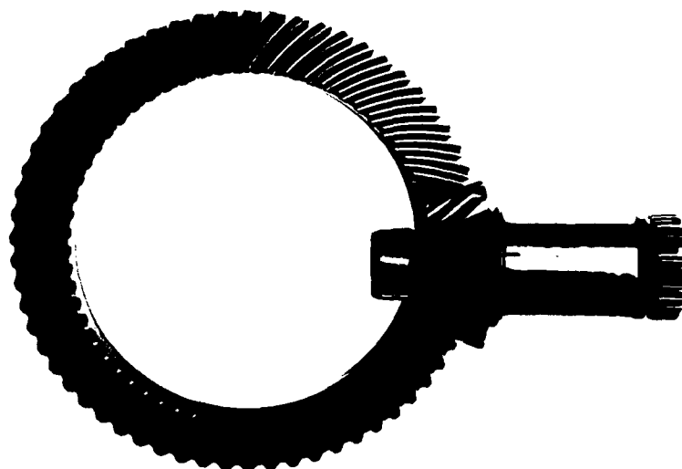
Figure 1. - Spiral-bevel gear and pinion.
