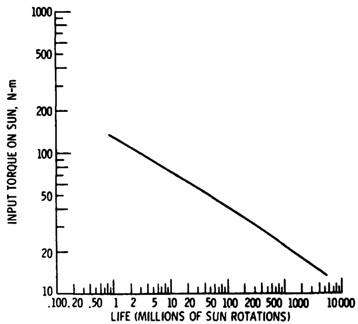
Figure 7. - Load-life curve for a full planetary system.
