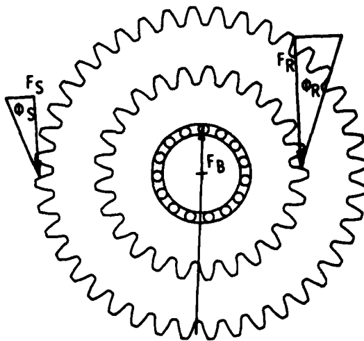
Figure 3. - Planet gear forces.
