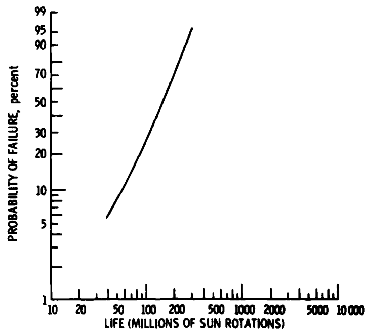
Figure 4. - Weibull graph of S_T versus L_T for a full planetary system.
