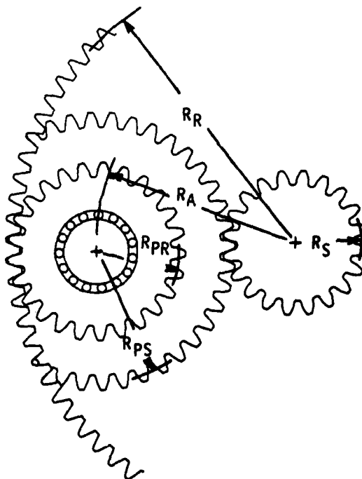
Figure 2. - Planetary geometry.
