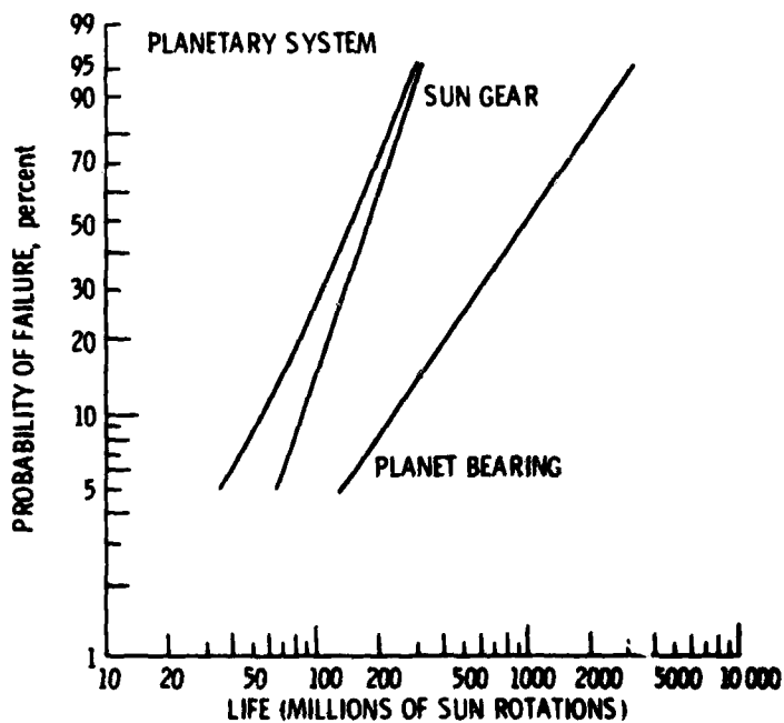
Figure 6. - Weibull graphs for sun gear, planet bearing, and transmission for a planetary with balanced components.
