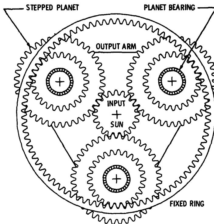
Figure 1. - Planetary gear train.
