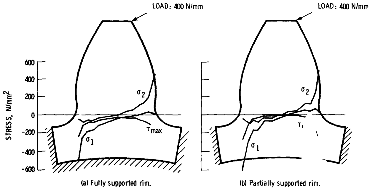
Figure 9. - Internal root section principal stresses with tip loading with a rim radius of 35mm.
