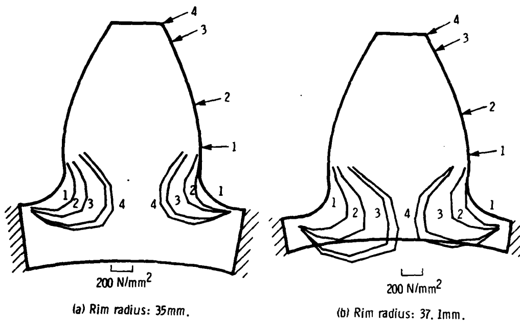
Figure 7. - Surface stress distribution at the fillet for a partially supported rim.
