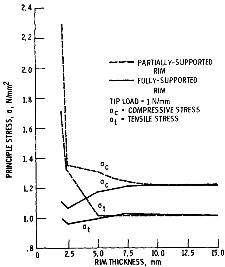
Figure 8. - Variation of maximum fillet stresses with rim thickness.
