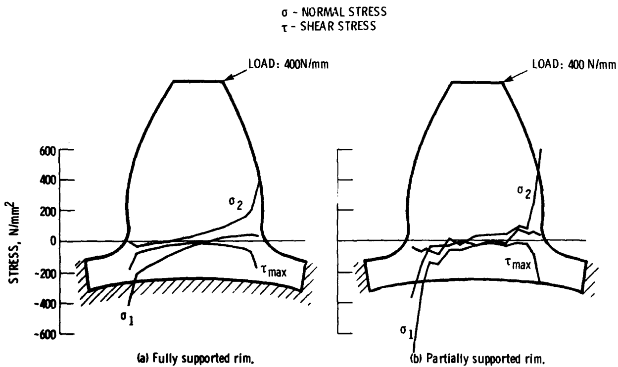
Figure 10. - Internal root section principal stresses with tip loading with a rim radius of 37.1mm.
