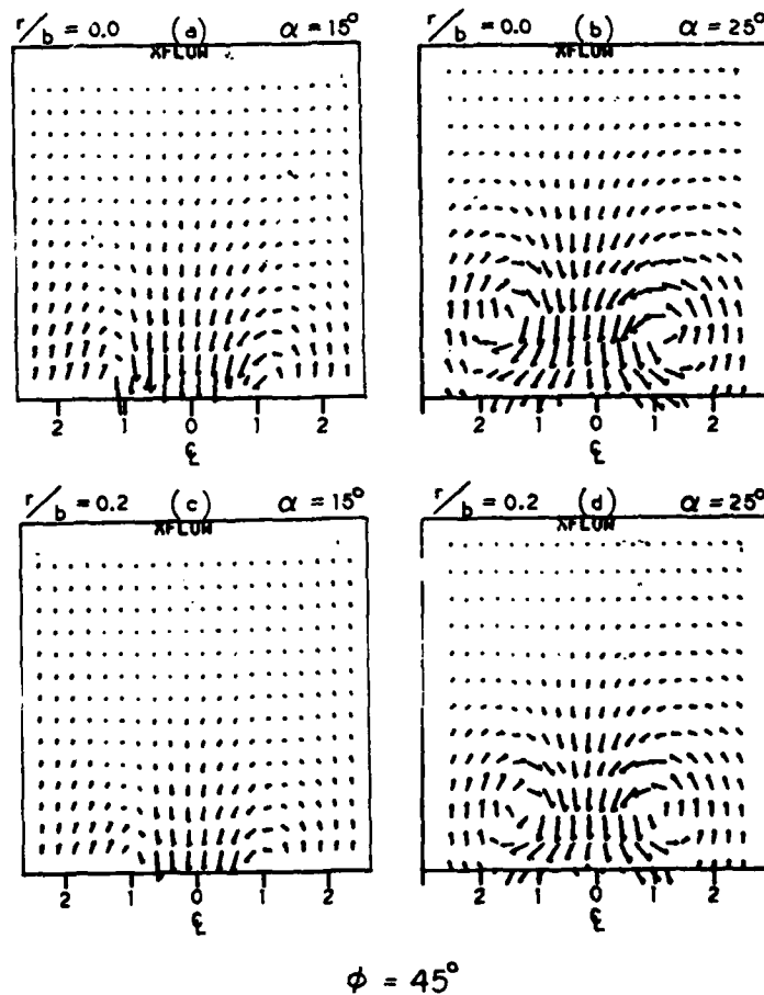
Figure 8. Velocity Patterns behind Two Body Cross-Sections (with Cross-Section Corner Radii of 0 Percent and 20 Percent) at Two Angles of Attack (15 Degrees and 25 Degrees) and a Roll Angle of 45 Degrees
