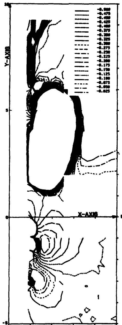
Figure 9: Total Pressure Coefficient Contours with Canard Z = +4 inches
