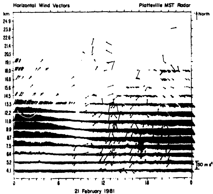
Figure 2. Horizontal wind vectors at Platteville. Basic time resolution is two and one half minutes.
