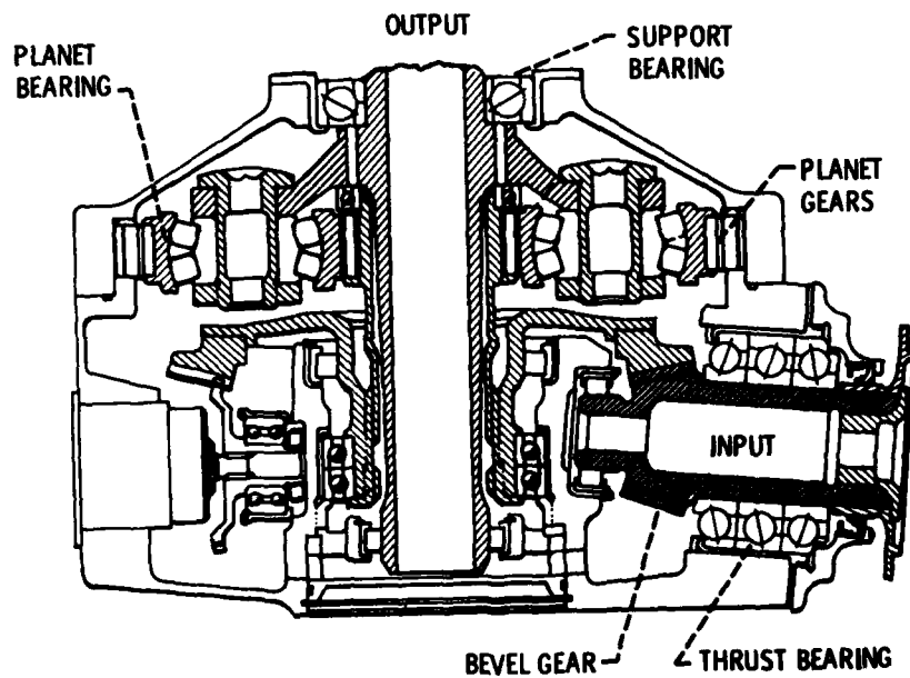
Figure 5. - Cross section of OH-58 helicopter transmission.
