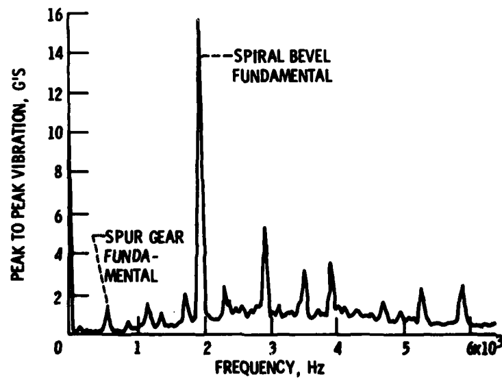
Figure 8. - Typical vibration spectrum.
