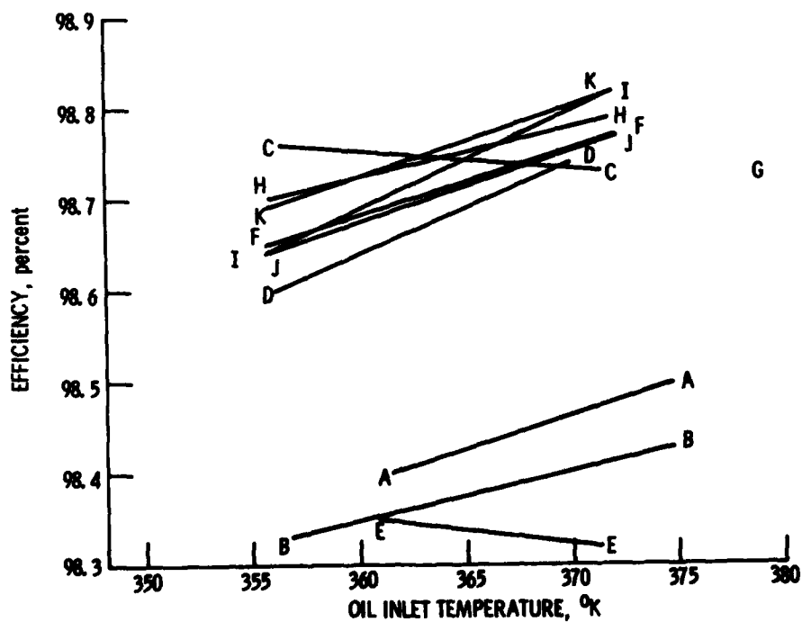
Figure 6. - Experimental efficiency correlated with inlet oil temperature.
