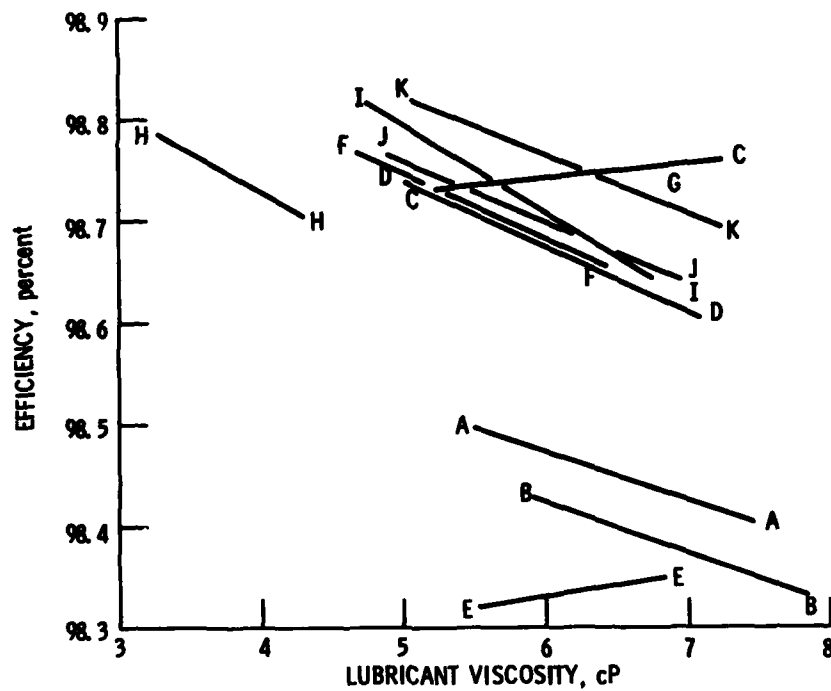
Figure 7. - Experimental efficiency correlated with lubricant viscosity.
