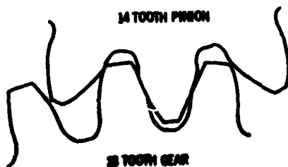
Figure 3. - Unequal addenda mesh geometry.
