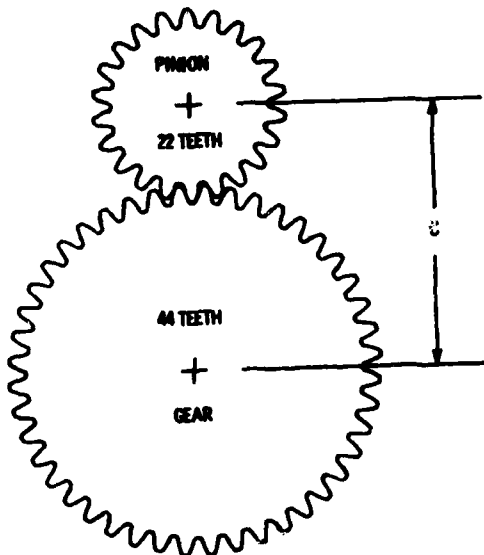
Figure 1. - Standard gear mesh.
