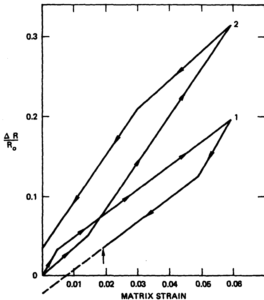
FIGURE 7 CALCULATED RESISTANCE CHANGE OF Yb GAUGE (MODELED AS ELASTIC-PLASTIC INCLUSIONS) VERSUS MATRIX STRAIN
