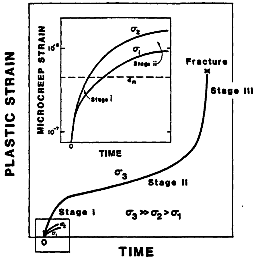
Figure 1 Schematic constant-load, constant temperature uniaxial creep record, showing the three major stages of creep. The inset is a schematic showing microcreep records for two stresses. Very small strains are measurable and distinguishable from one another when the strain reaches the minimum detectable limit of the strain measuring equipment, which is designated \epsilon_m in the inset.
