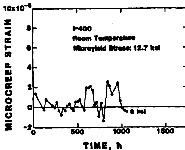
Figure 2 Some typical microcreep test records on I-400 beryllium from the literature.
