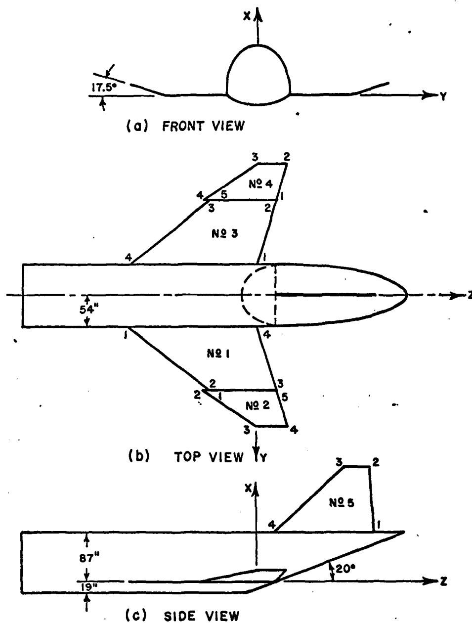
Fig. 54. Illustration of geometry of F-4 aircraft model used in finite elliptic cylinder model.
