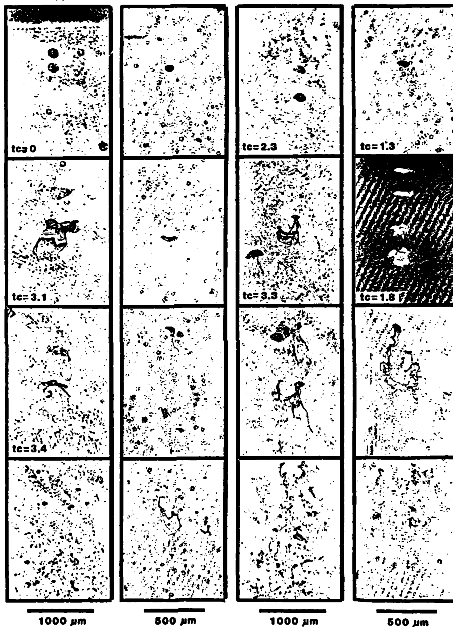
FIGURE 6. Weber Number Effects on Ethanol Droplet Breakup
