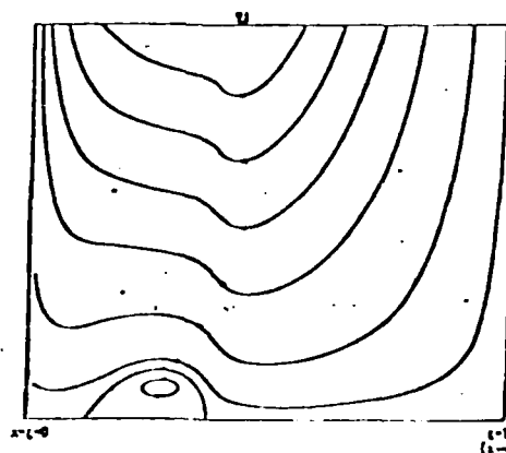
Figure 13. Boundary layer streamlines due to a downward moving pair started at X_0=3.28 , Y_0=1.05 at t=1.225 .
