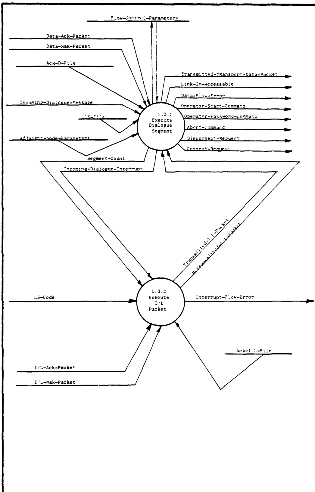
Figure C-16 Execute Incoming Dialogue Message (1.3) DFD
