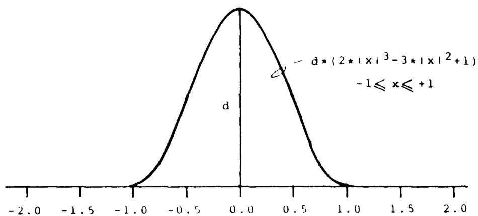
Akima Interpolation Impulse Response
